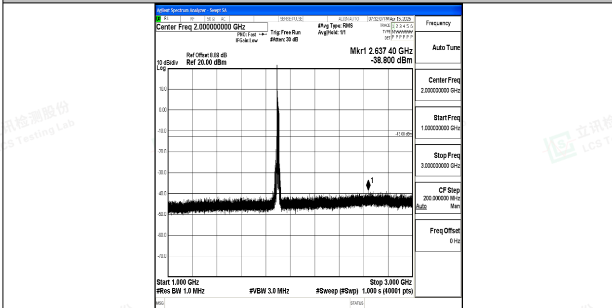
Band2_20MHz_16QAM_19100_1RB#0_1000~3000_1000~3000
