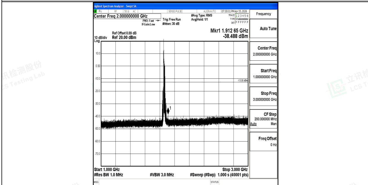
Band2_20MHz_16QAM_18700_1RB#0_1000~3000_1000~3000
