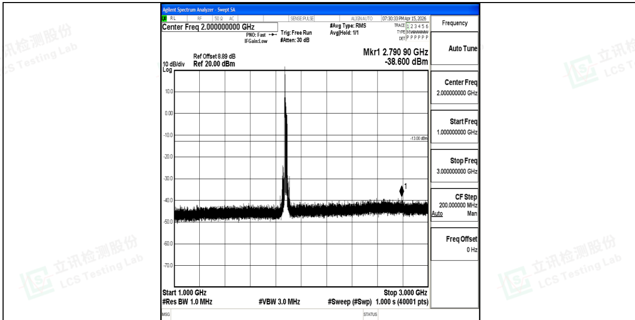
Band2_20MHz_QPSK_18900_1RB#0_1000~3000_1000~3000
