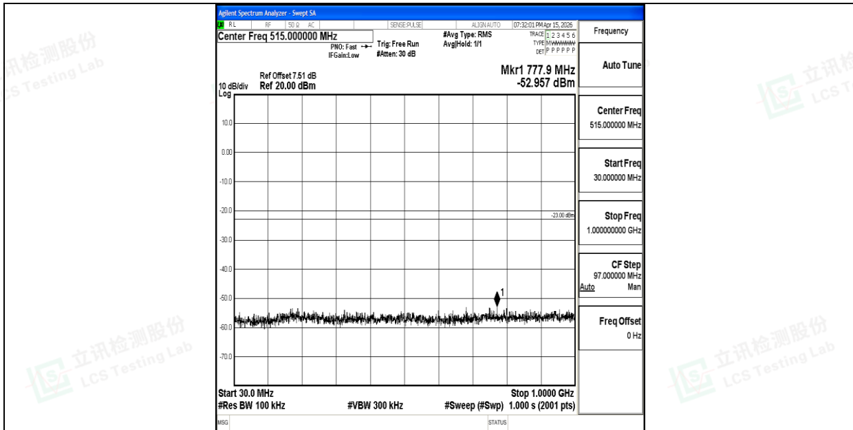
Band2_20MHz_16QAM_19100_1RB#0_30~1000_30~1000
