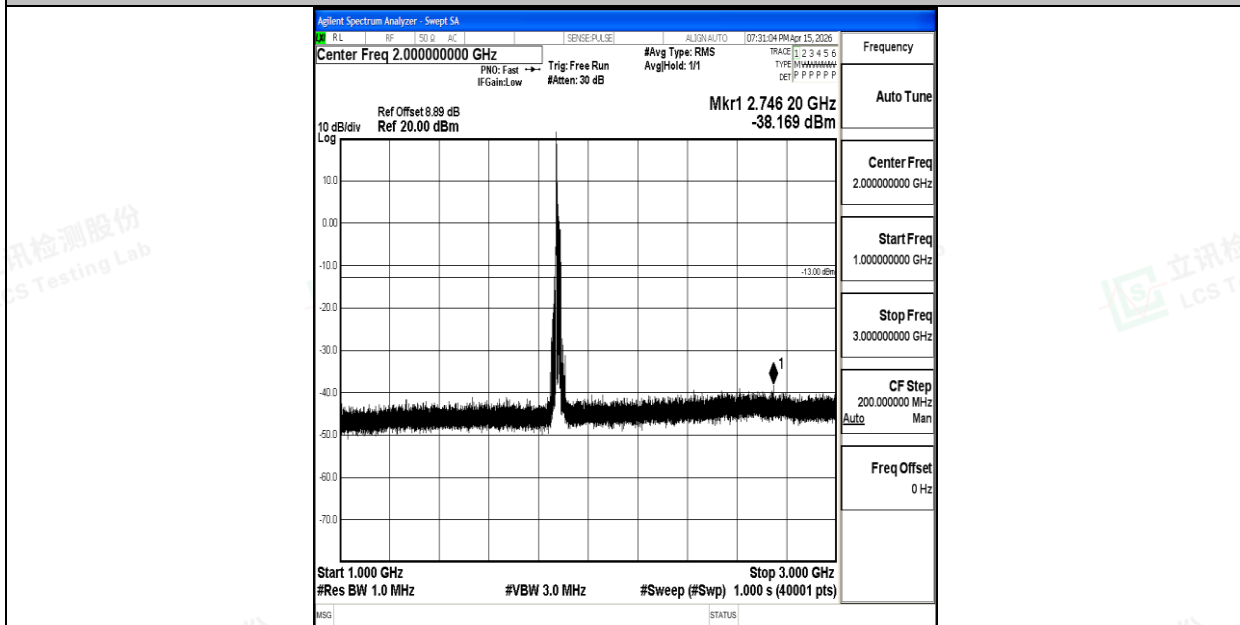
Band2_20MHz_16QAM_18900_1RB#0_1000~3000_1000~3000
