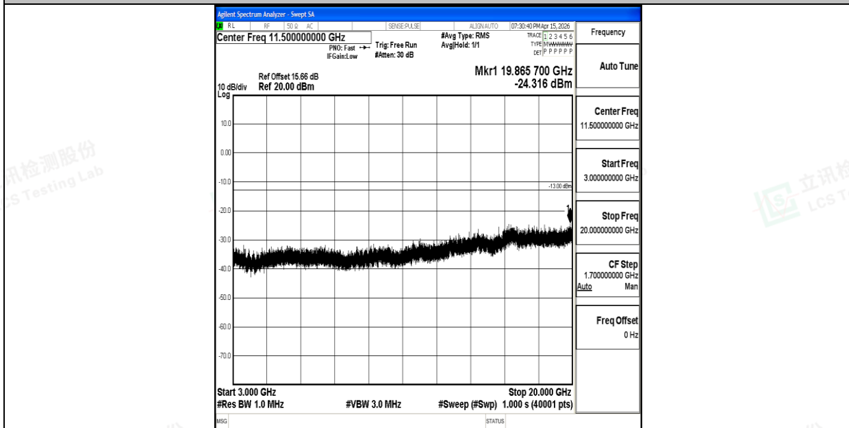
Band2_20MHz_QPSK_18900_1RB#0_3000~20000_3000~20000
