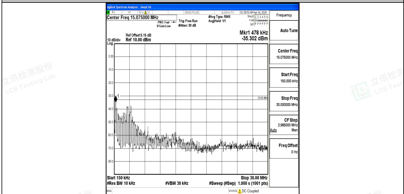
Band25_1.4MHz_16QAM_26047_1RB#0_0.15~30_0.15~30
