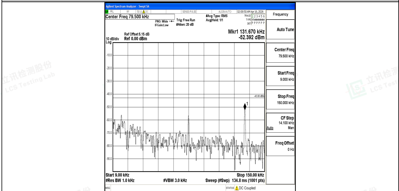
Band25_3MHz_QPSK_26055_1RB#0_0.009~0.15_0.009~0.15
