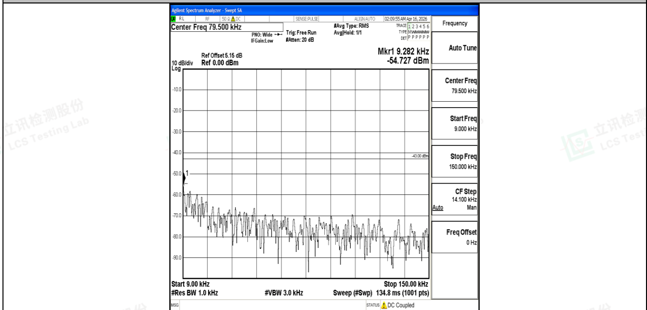
Band25_3MHz_QPSK_26365_1RB#0_0.009~0.15_0.009~0.15
