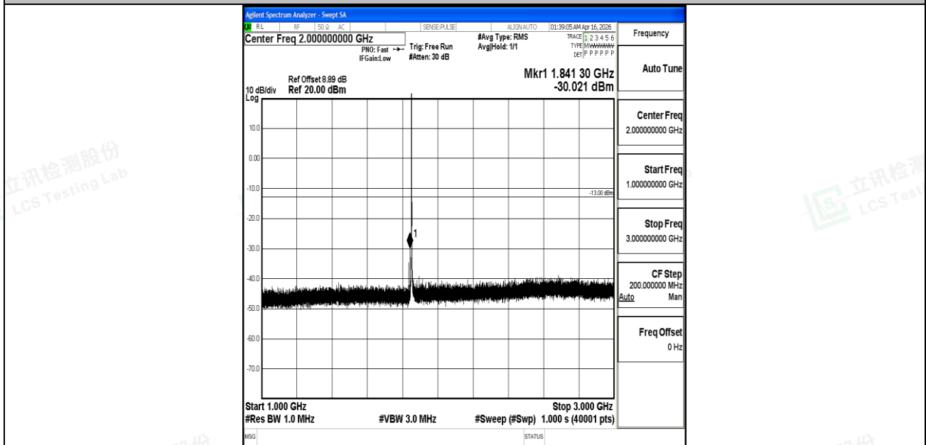
Band25_1.4MHz_16QAM_26047_1RB#0_1000~3000_1000~3000
