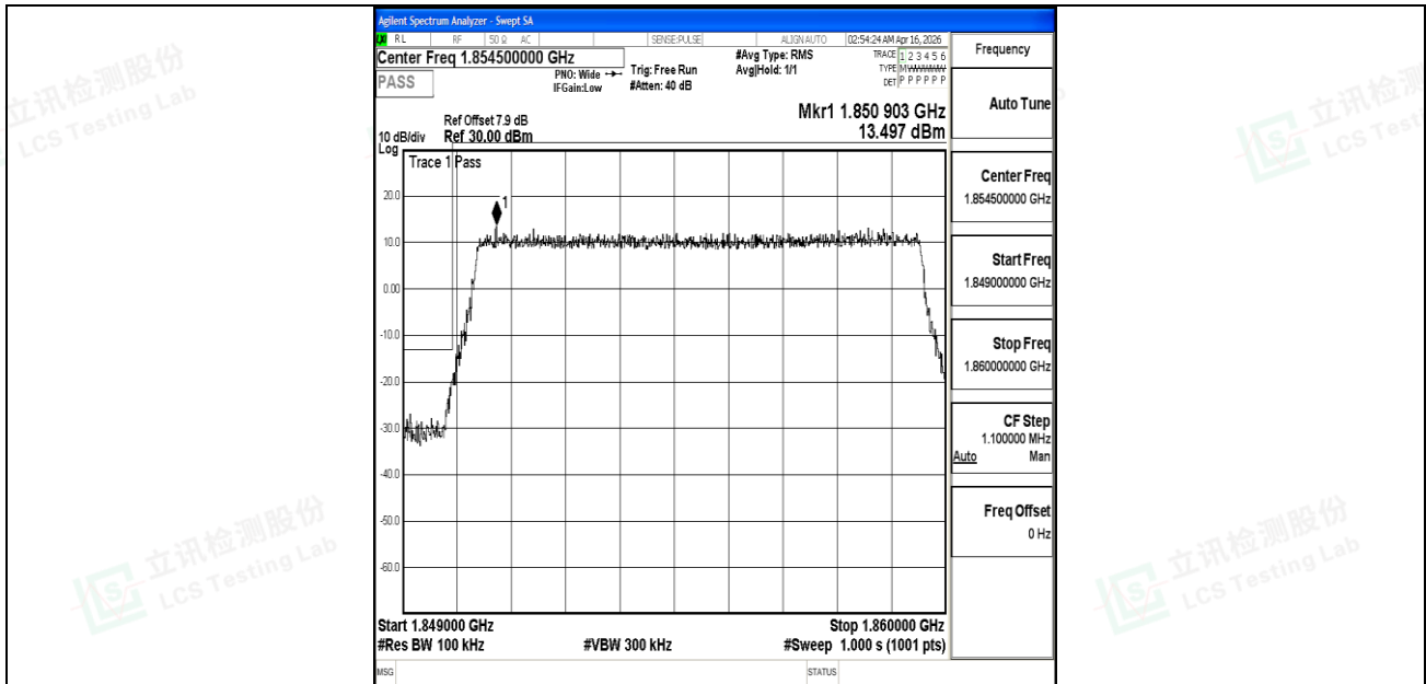
Band25_10MHz_QPSK_26090_50RB#0
