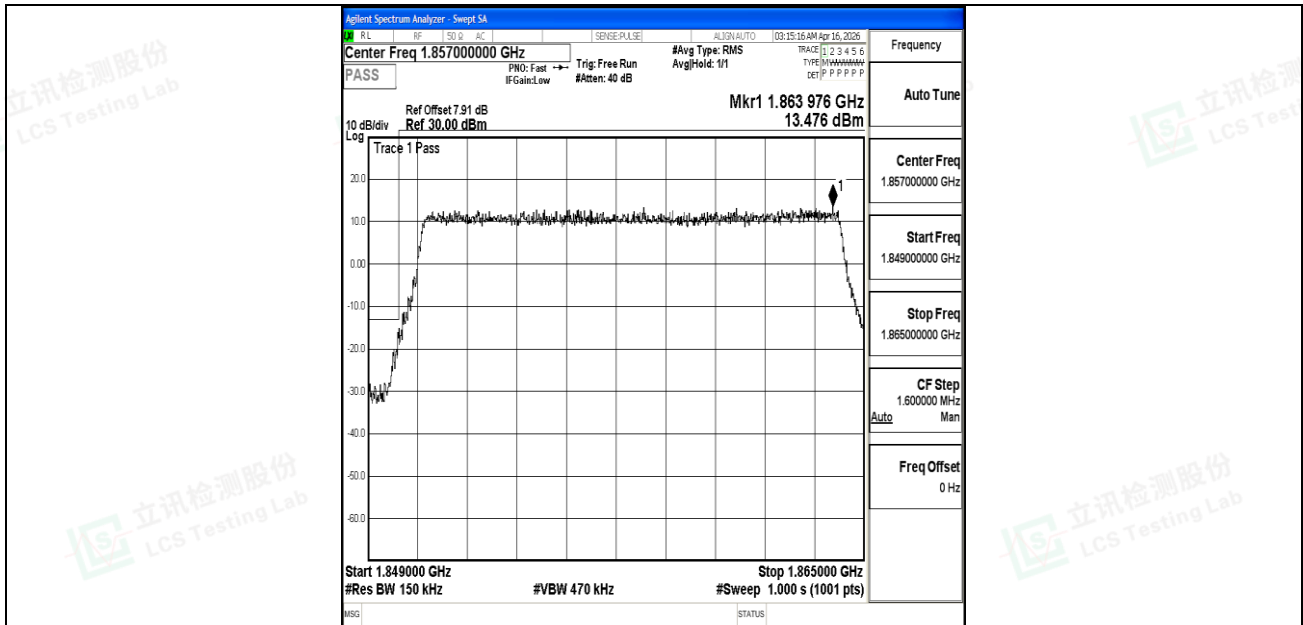
Band25_15MHz_QPSK_26115_75RB#0
