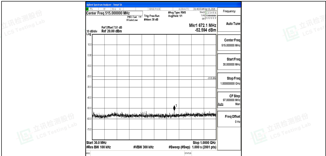
Band25_1.4MHz_16QAM_26365_1RB#0_30~1000_30~1000
