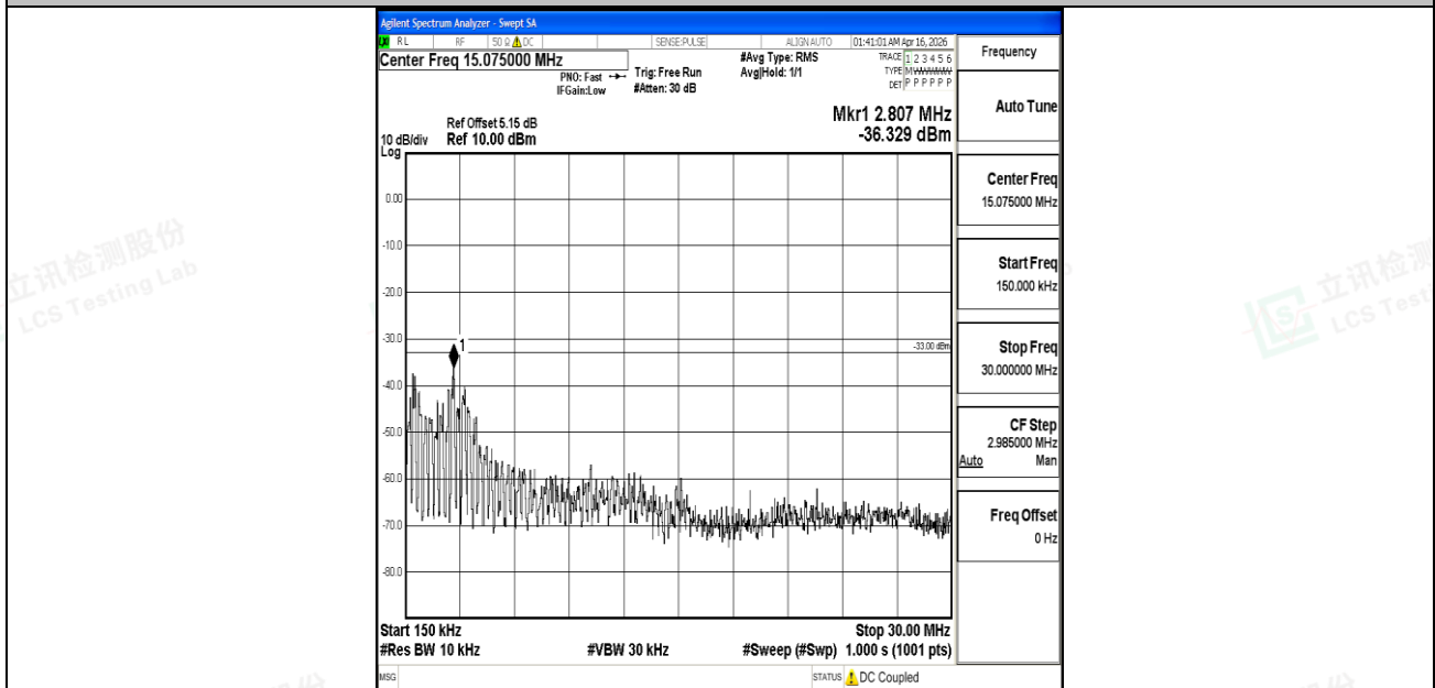
Band25_1.4MHz_16QAM_26683_1RB#0_0.15~30_0.15~30
