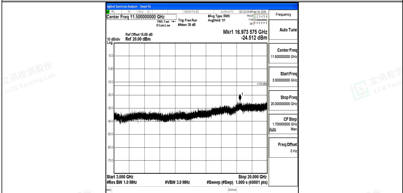
Band25_3MHz_QPSK_26365_1RB#0_3000~20000_3000~20000
