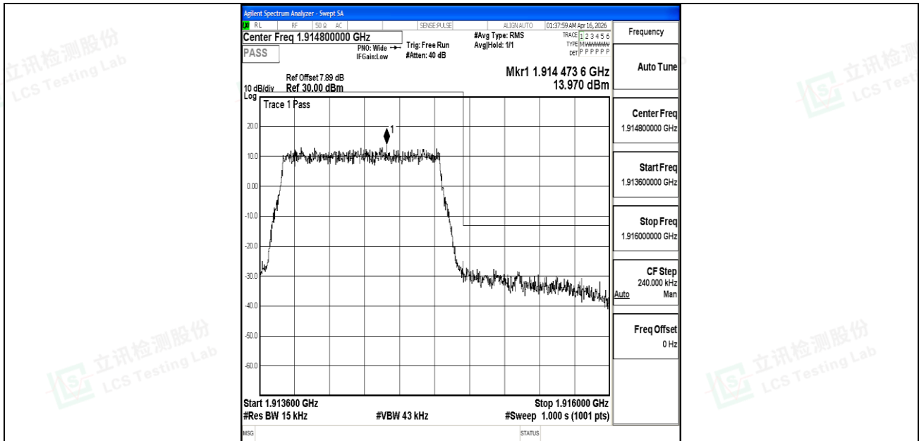
Band25_1.4MHz_QPSK_26683_6RB#0
