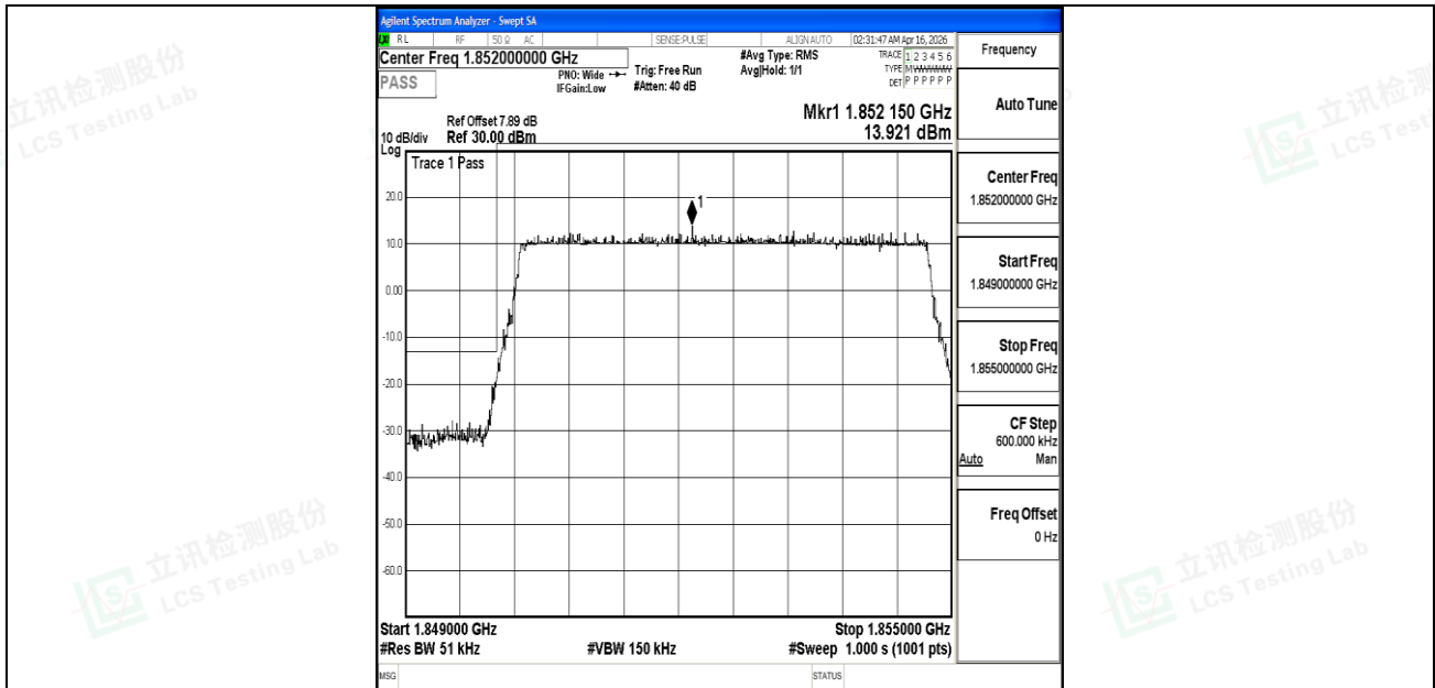
Band25_5MHz_QPSK_26065_25RB#0
