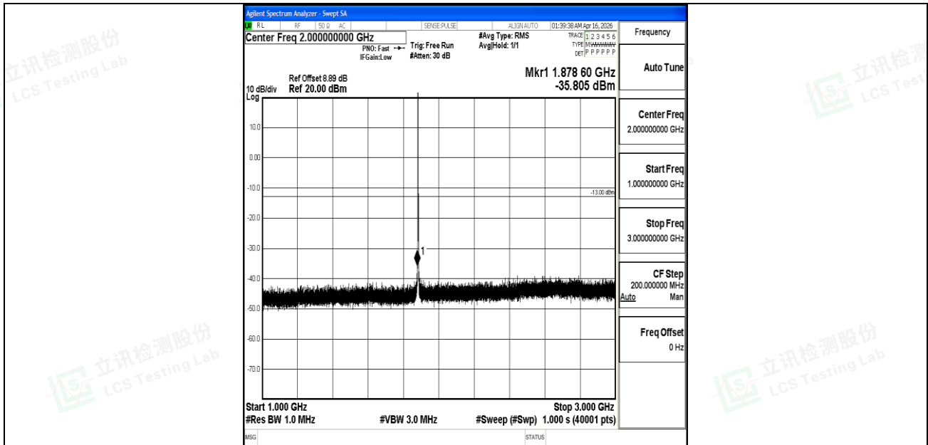
Band25_1.4MHz_QPSK_26365_1RB#0_1000~3000_1000~3000
