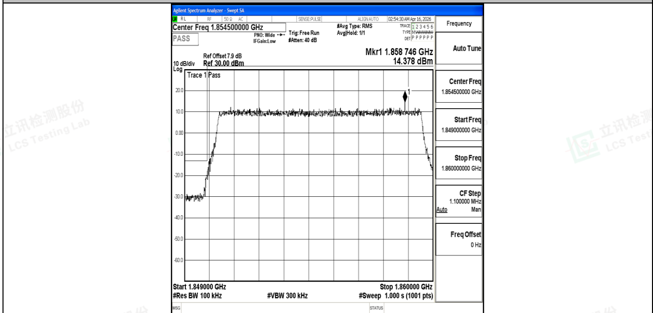
Band25_10MHz_16QAM_26090_50RB#0
