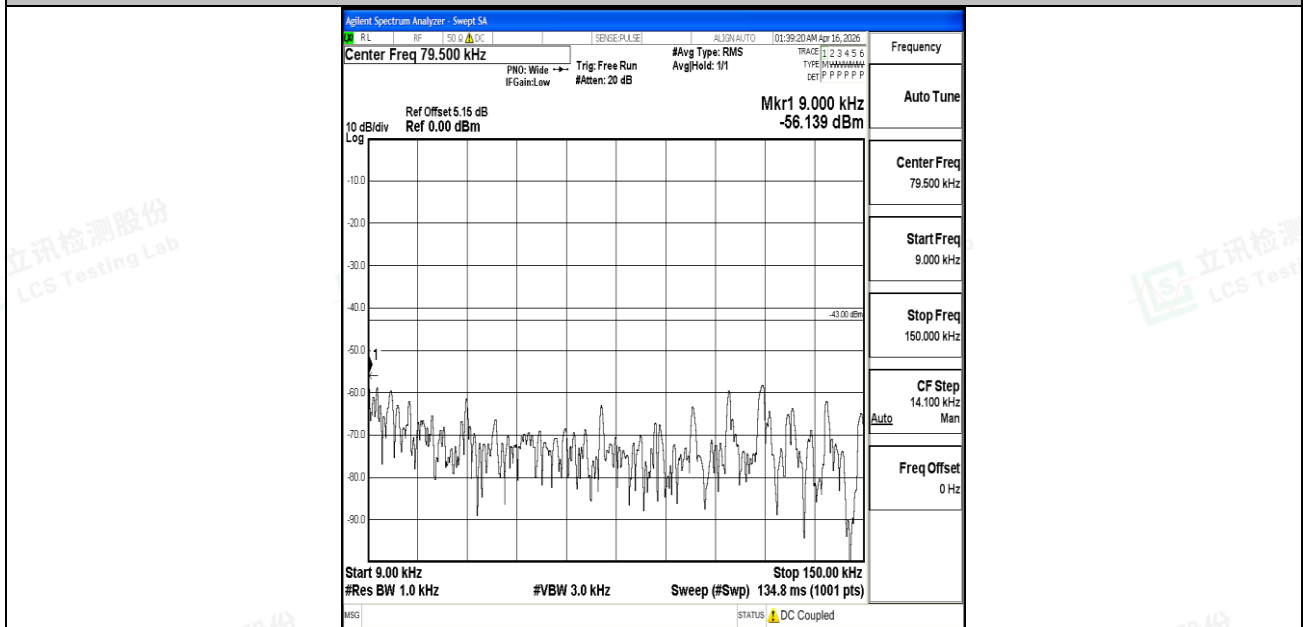
Band25_1.4MHz_QPSK_26365_1RB#0_0.009~0.15_0.009~0.15
