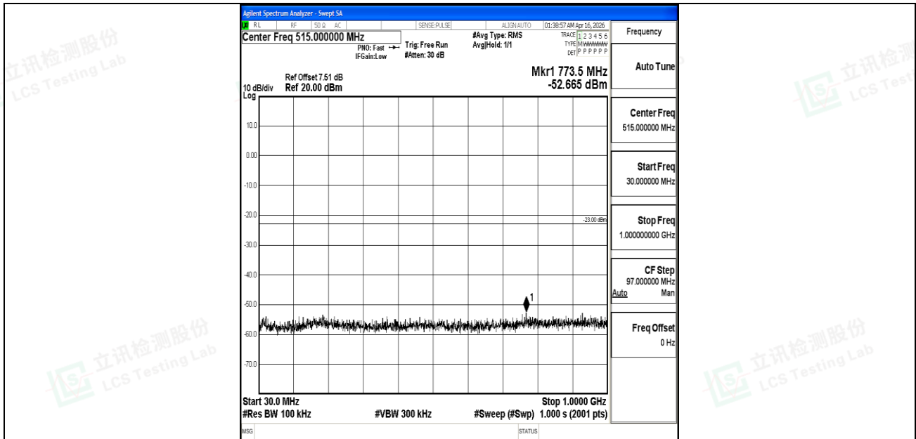
Band25_1.4MHz_16QAM_26047_1RB#0_30~1000_30~1000
