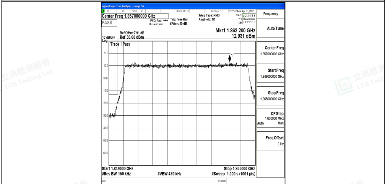
Band25_15MHz_16QAM_26115_75RB#0
