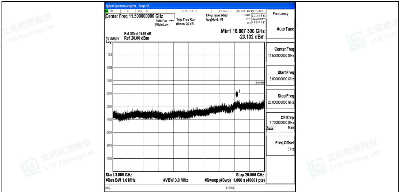
Band25_1.4MHz_16QAM_26047_1RB#0_3000~20000_3000~20000
