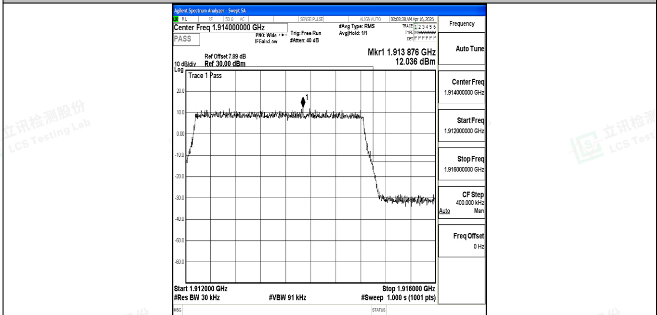
Band25_3MHz_16QAM_26675_15RB#0
