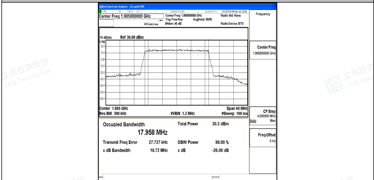
Band25-20MHz-16QAM-26590-100RB#0-PASS
