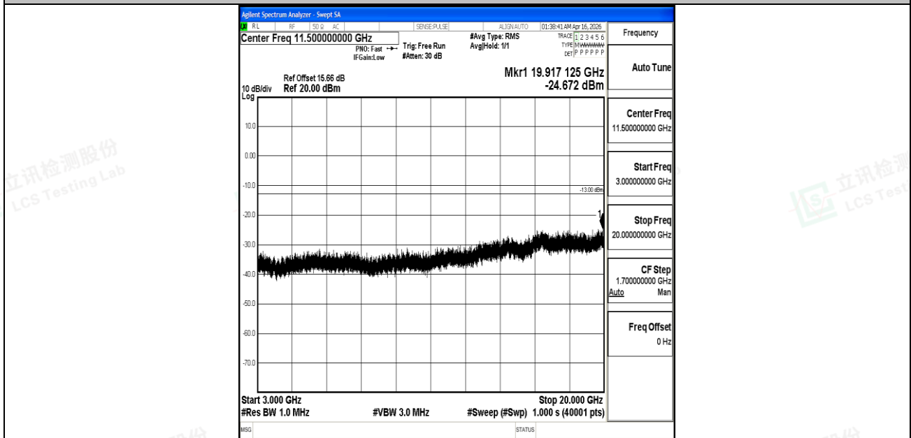
Band25_1.4MHz_QPSK_26047_1RB#0_3000~20000_3000~20000
