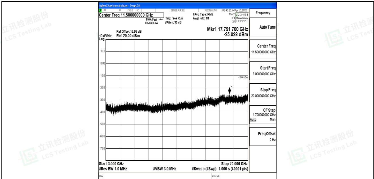
Band25_1.4MHz_16QAM_26365_1RB#0_3000~20000_3000~20000
