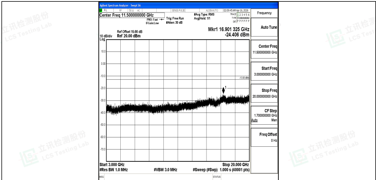
Band25_3MHz_16QAM_26055_1RB#0_3000~20000_3000~20000
