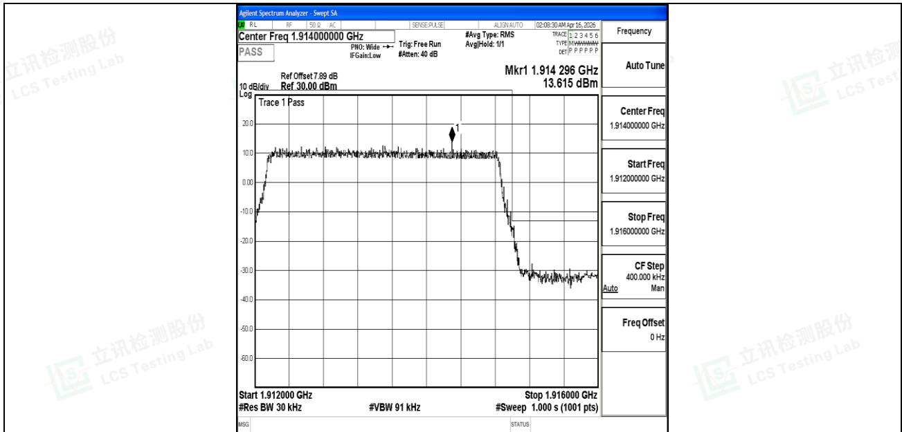
Band25_3MHz_QPSK_26675_15RB#0
