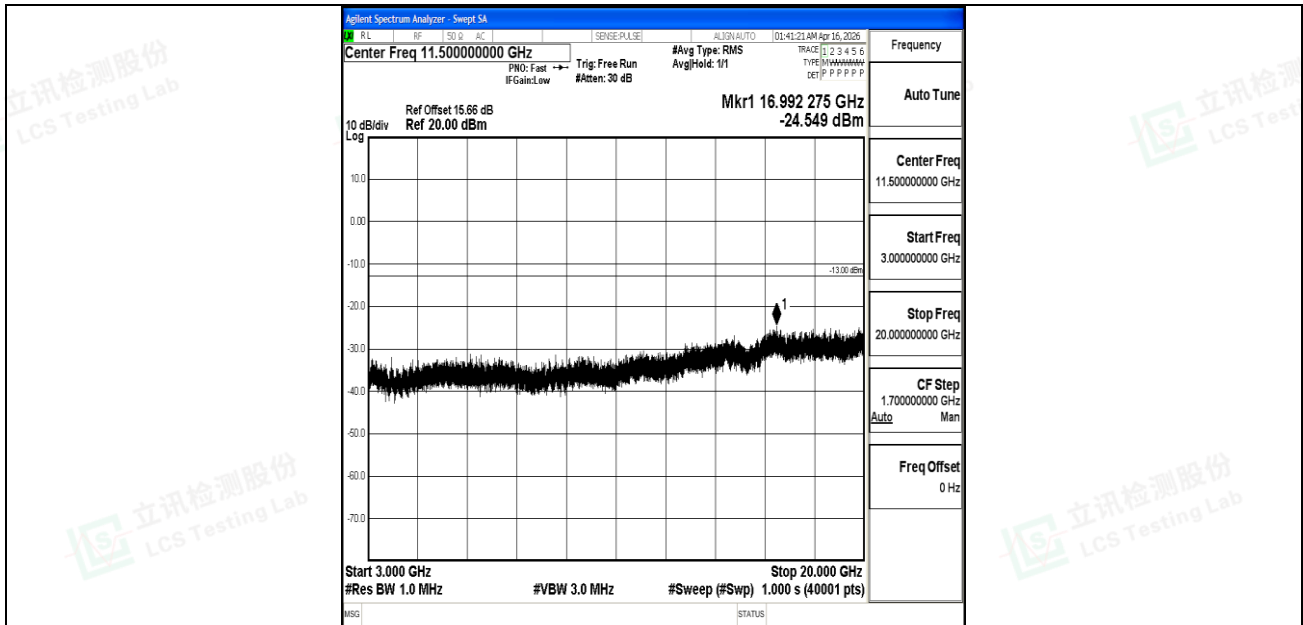
Band25_1.4MHz_16QAM_26683_1RB#0_3000~20000_3000~20000
