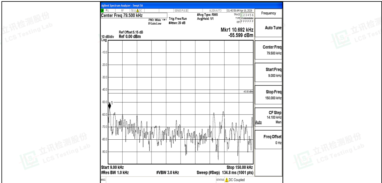
Band25_1.4MHz_16QAM_26683_1RB#0_0.009~0.15_0.009~0.15
