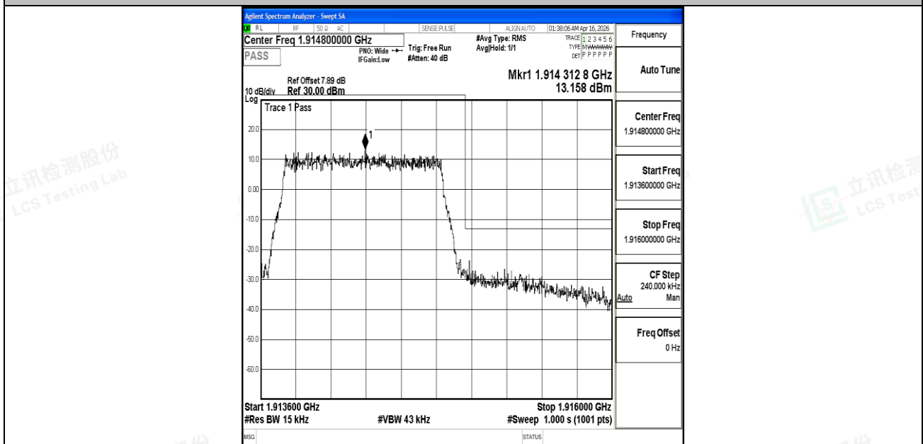
Band25_1.4MHz_16QAM_26683_6RB#0
