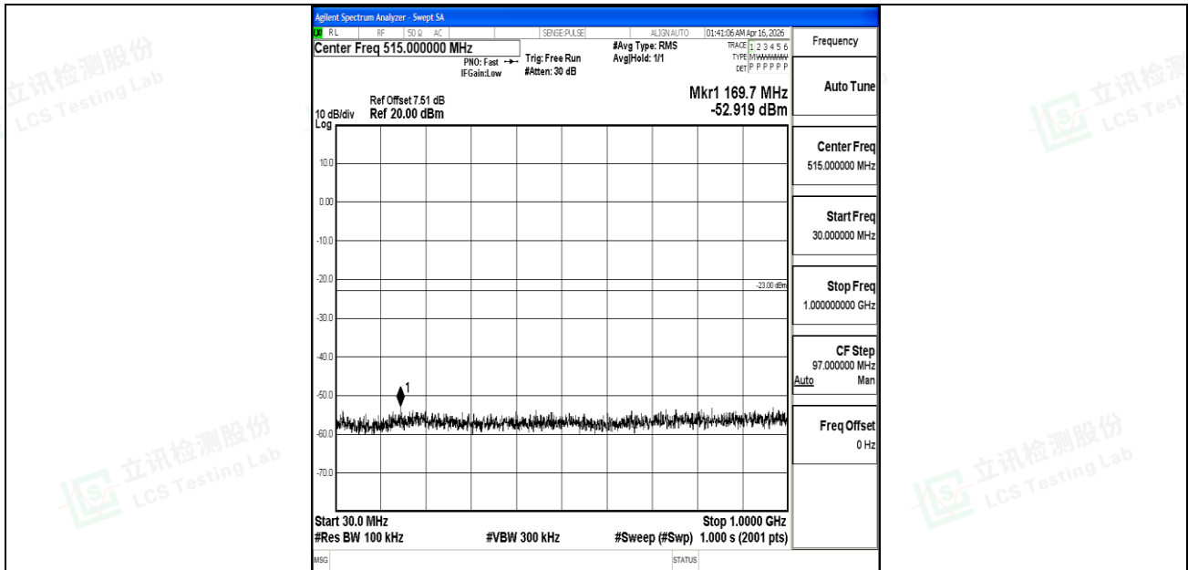
Band25_1.4MHz_16QAM_26683_1RB#0_30~1000_30~1000
