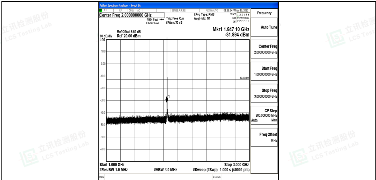
Band25_1.4MHz_QPSK_26047_1RB#0_1000~3000_1000~3000
