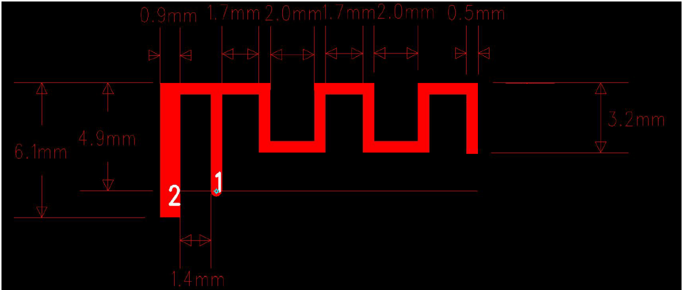
Antenna Photo & Length (mm)
