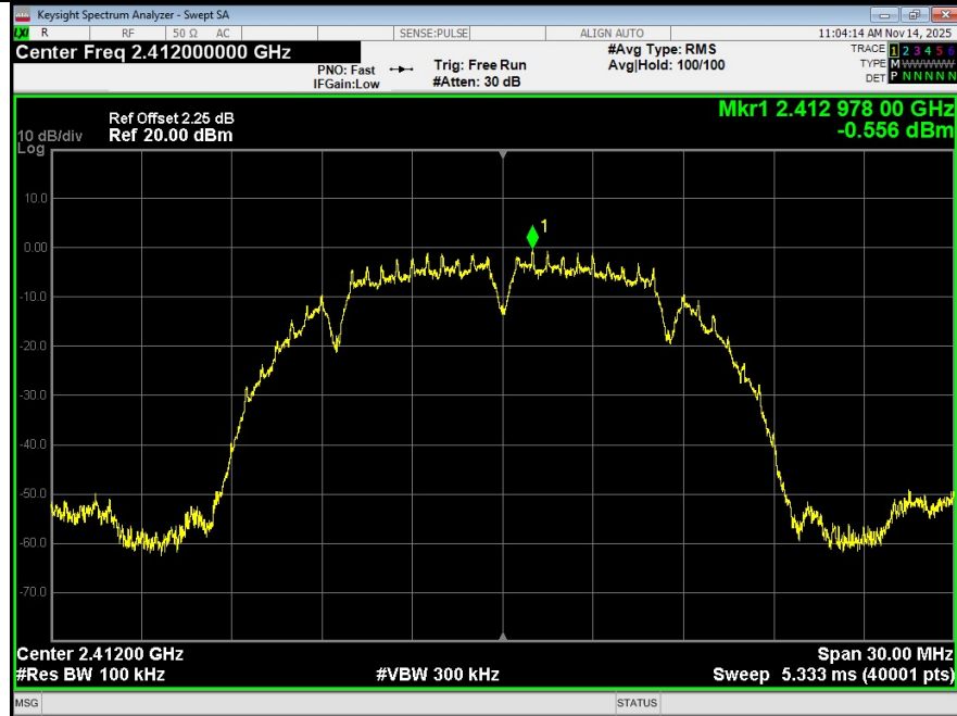
2_Bandedge_NVNT_ANT1_802_11b_2412
