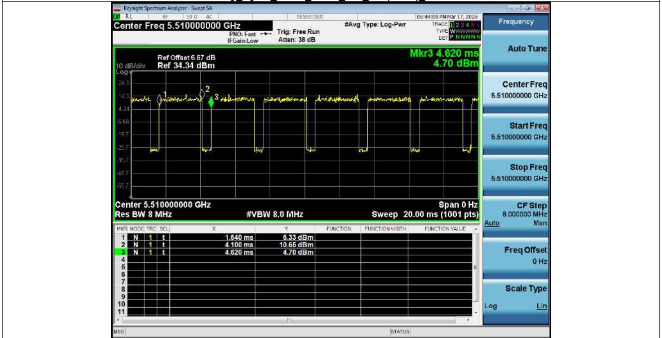
Duty_Cycle_NVNT_ANT1_802_11n(HT40)_5510
