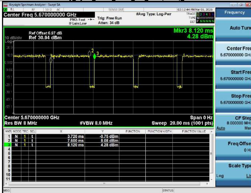
Duty Cycle_NVNT_ANT1_802_11ax(HE40)_5670
