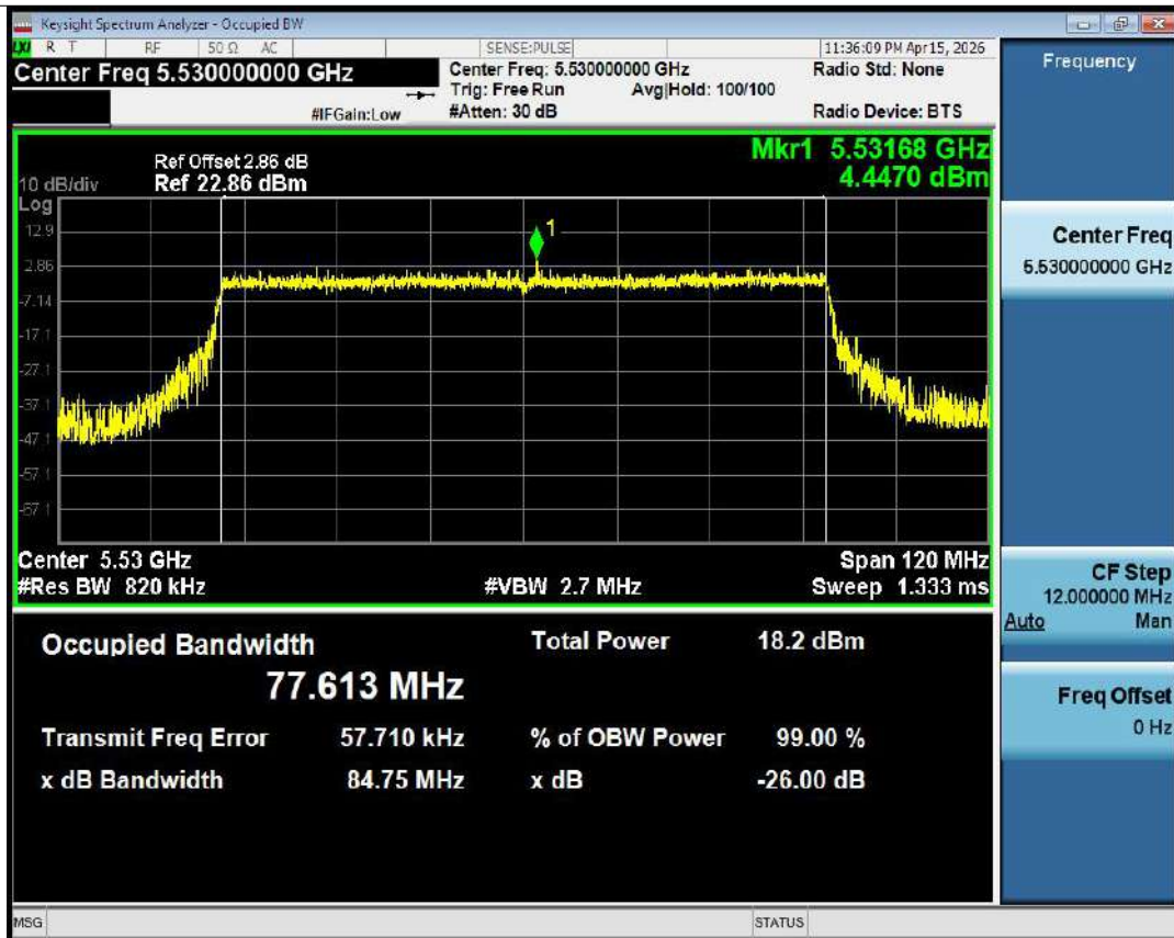
OBW NVNT ax80 5530MHz Ant1
