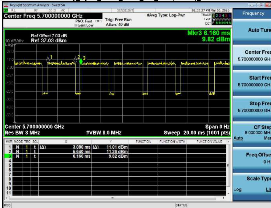
Duty Cycle NVNT ANT1 802_11ac(VHT20) 5700
