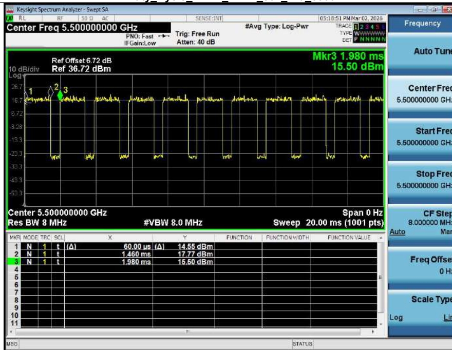
Duty Cycle NVNT_ANT1_802_11a_5500
