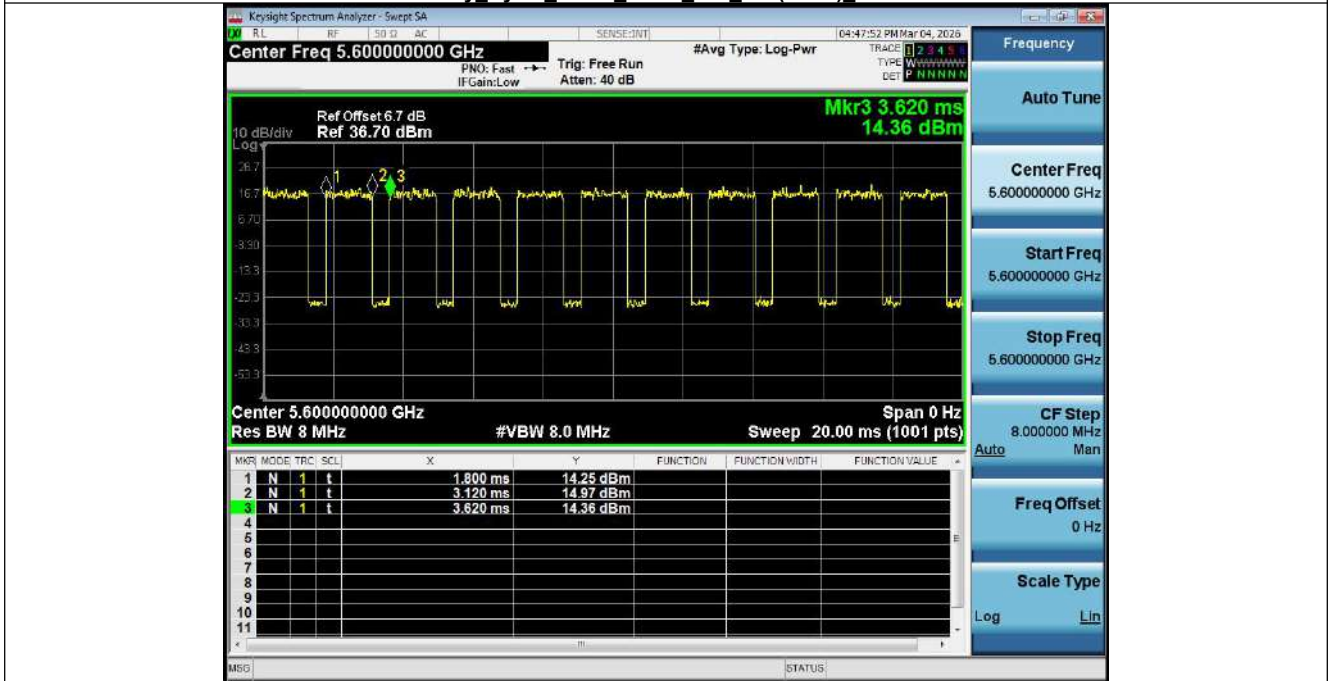
Duty_Cycle_NVNT_ANT1_802_11n(HT20)_5600
