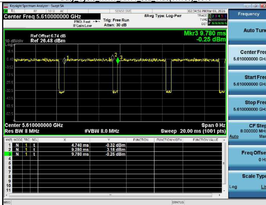
Duty_Cycle_NVNT_ANT1_802_11ac(VHT80)_5610
