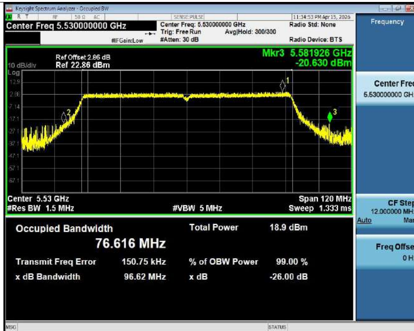
-26dB Bandwidth NVNT ac80 5530MHz Ant1
