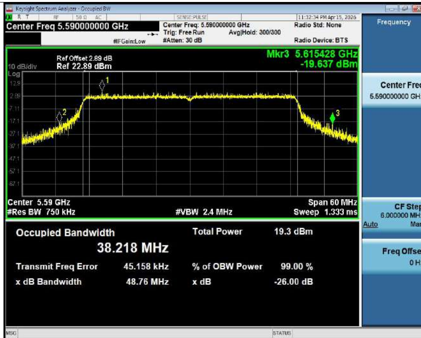
-26dB Bandwidth NVNT ax40 5590MHz Ant1
