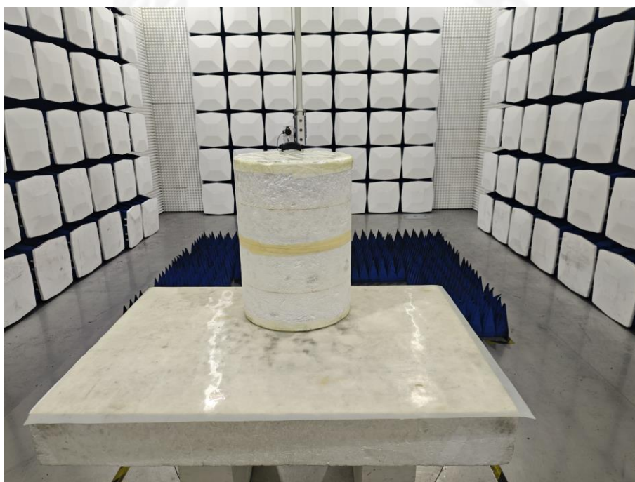
RE (18GHz-40GHz)
