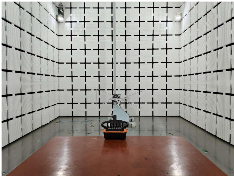
Radiated Emission Test View 1
