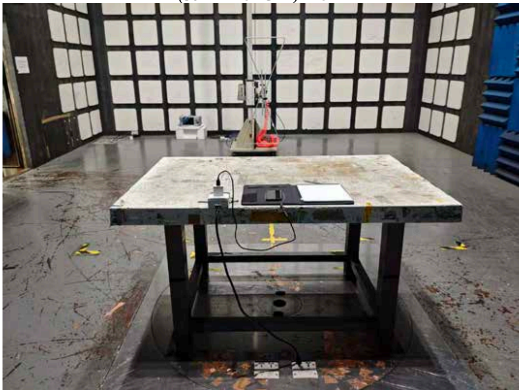
(30MHz TO 1GHz) BACK
