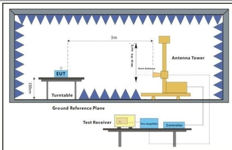
Figure 3. Above 1 GHz
