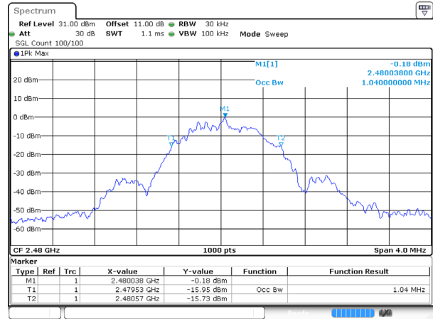
BLE (1 Mbps): High Channel
