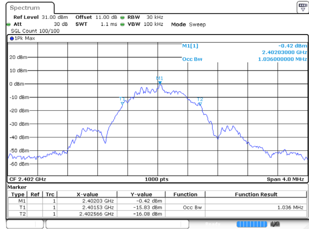
BLE (1 Mbps): Low Channel
