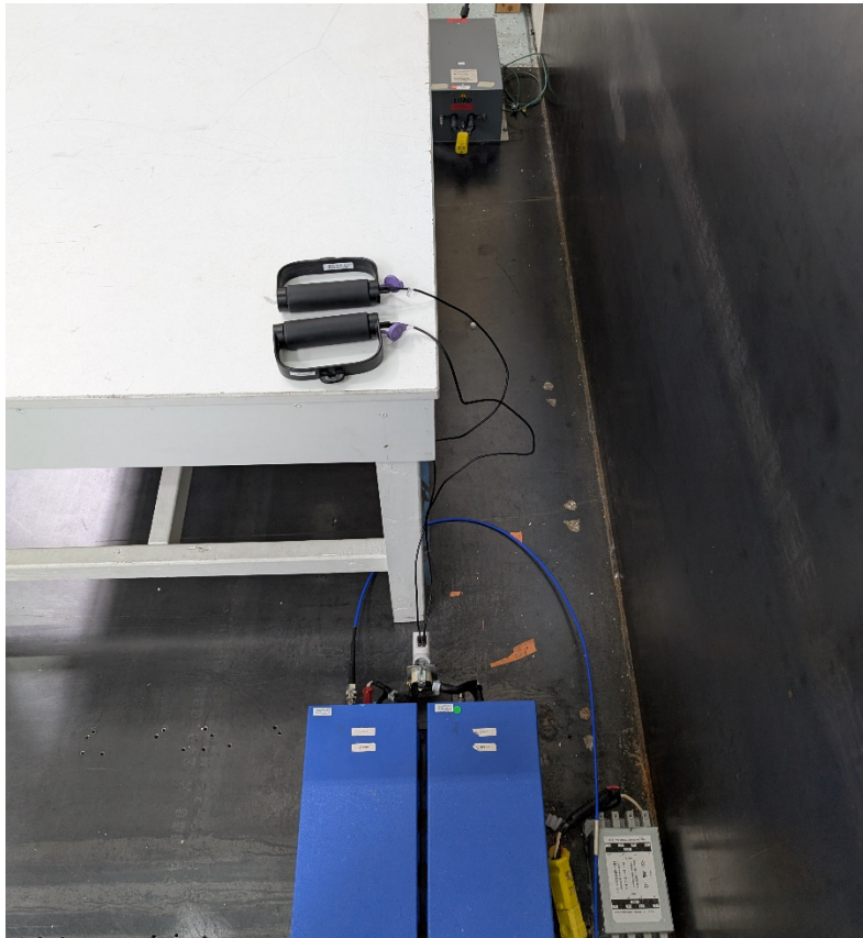
AC Power line Conducted Test Setup 2
