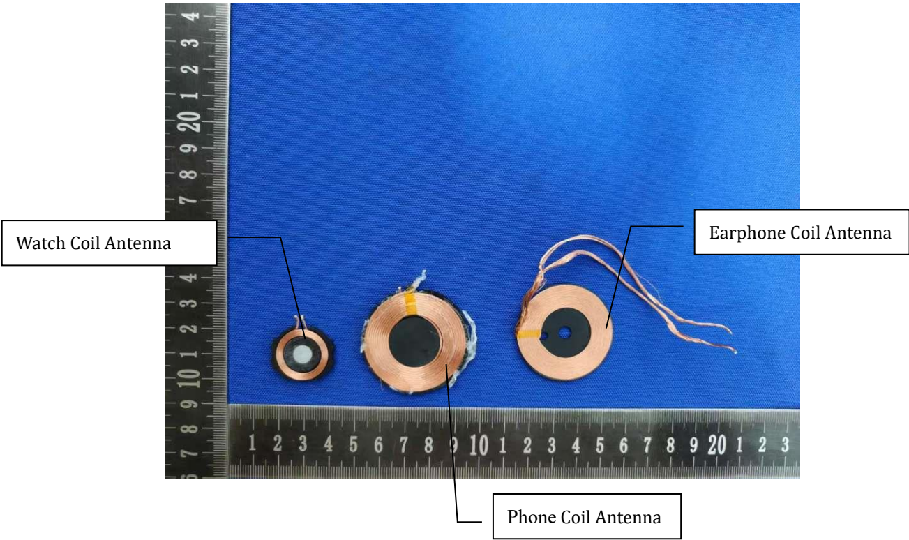
EUT Internal View 6
