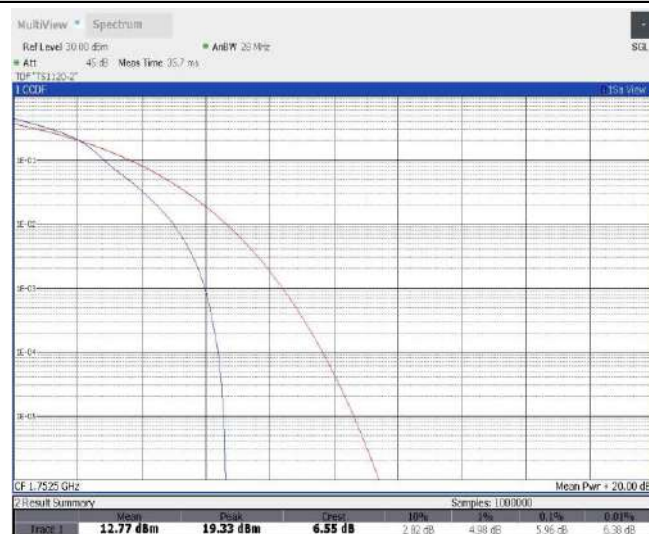
Band4-5MHz-16QAM-20375-25RB#0
