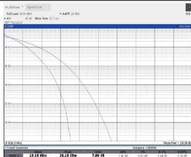
Band5-5MHz-QPSK-20525-1RB#0
