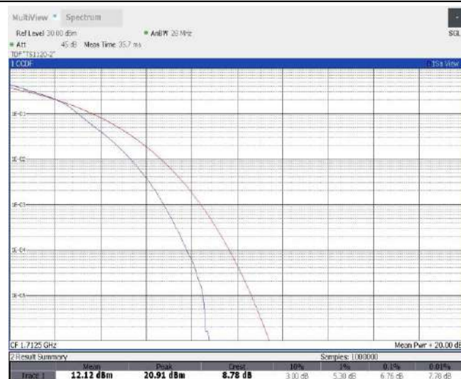
Band4-5MHz-16QAM-20175-1RB#0
