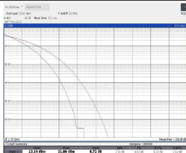
Band4-20MHz-QPSK-20175-1RB#0
