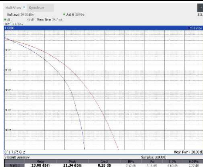
Band4-15MHz-QPSK-20175-1RB#0
