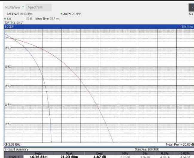
Band30-10MHz-16QAM-27710-1RB#0
