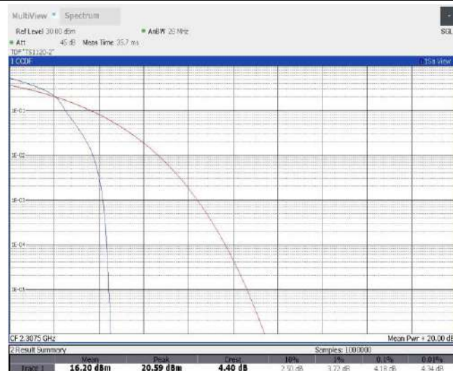
Band30-5MHz-16QAM-27685-25RB#0
