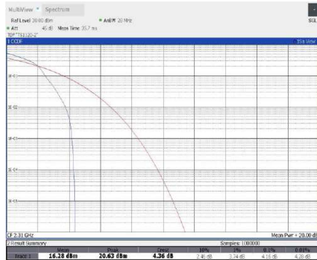
Band30-10MHz-16QAM-27710-50RB#0
