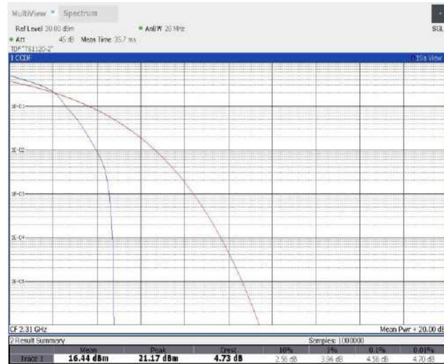
Band30-5MHz-16QAM-27710-25RB#0
