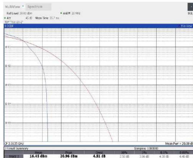
Band30-5MHz-16QAM-27735-25RB#0
