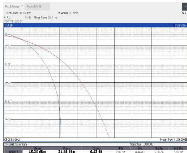
Band30-5MHz-16QAM-27735-1RB#0
