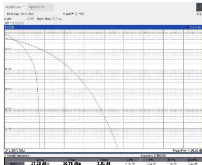
Band30-5MHz-QPSK-27685-25RB#0
