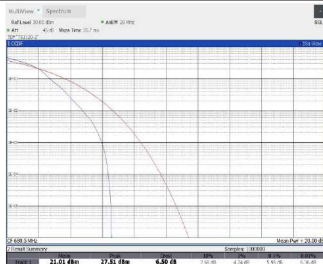
Band71-5MHz-16QAM-133297-25RB#0
