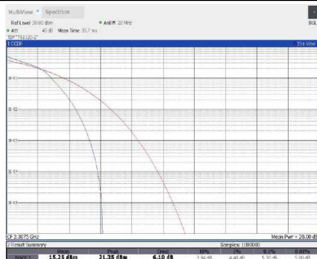
Band30-5MHz-16QAM-27710-1RB#0
