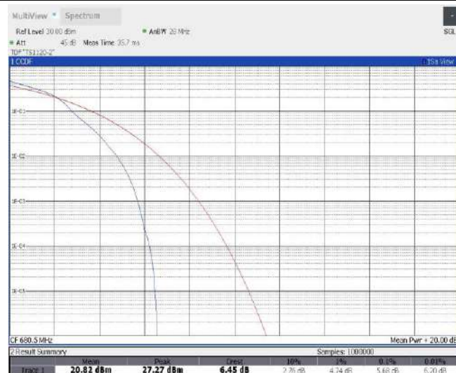
Band71-10MHz-16QAM-133297-50RB#0
