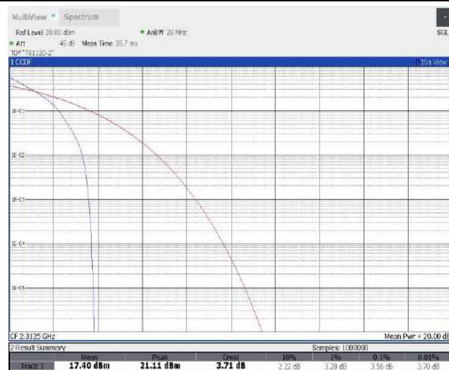
Band30-5MHz-QPSK-27735-25RB#0
