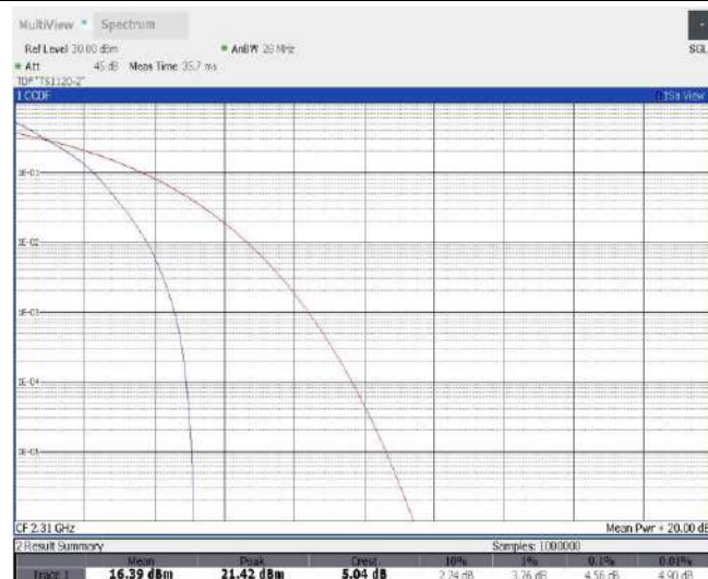
Band30-5MHz-QPSK-27735-1RB#0
