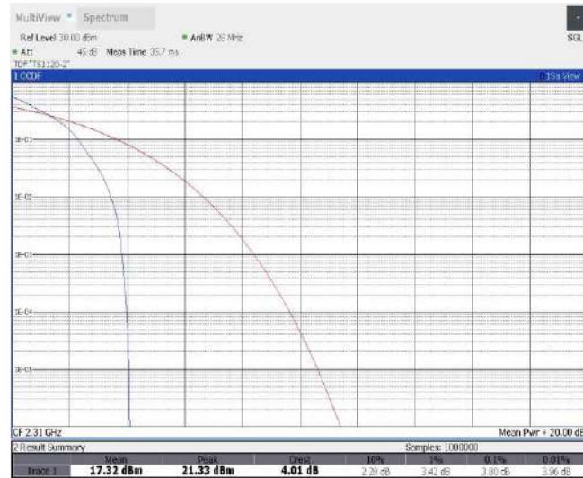
Band30-5MHz-QPSK-27710-25RB#0
