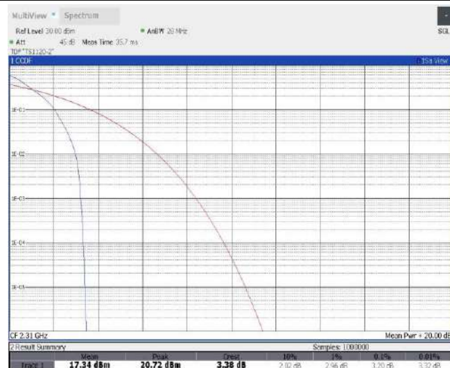
Band30-10MHz-QPSK-27710-50RB#0
