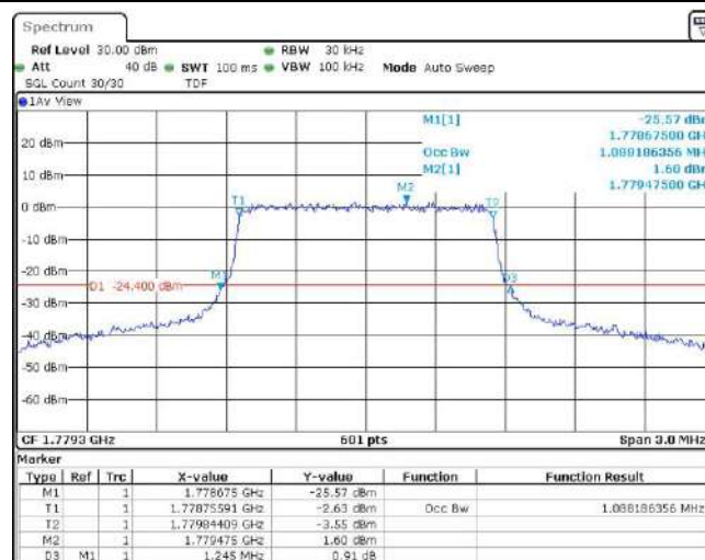
Band66-1.4MHz-16QAM-131979-6RB#0
