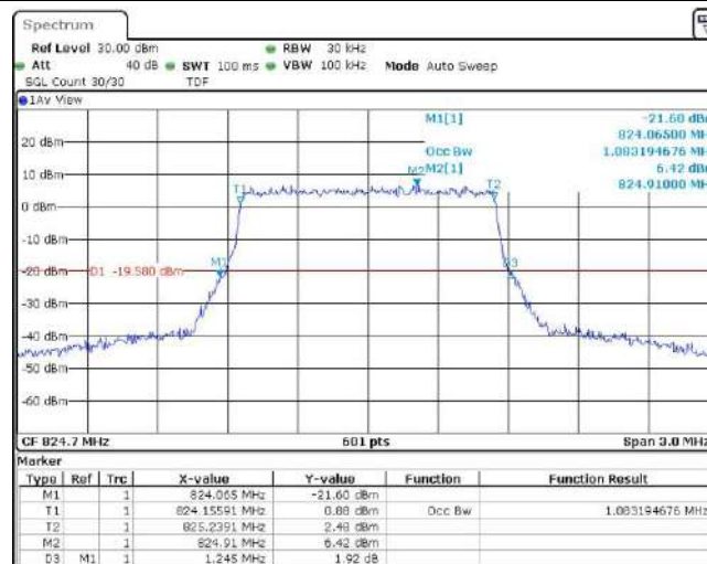
Band5-1.4MHz-16QAM-20525-6RB#0
