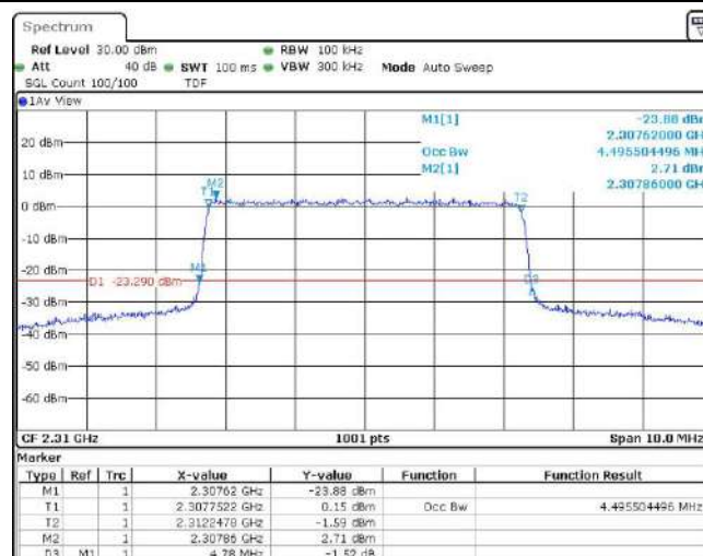
Band30-5MHz-16QAM-27735-25RB#0
