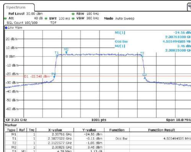
Band30-5MHz-QPSK-27735-25RB#0
