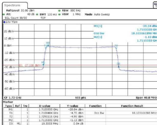
Band66-20MHz-16QAM-132322-100RB#0
