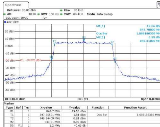
Band5-3MHz-QPSK-20415-15RB#0
