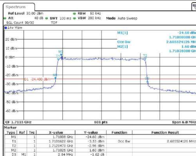
Band4-3MHz-QPSK-20175-15RB#0
