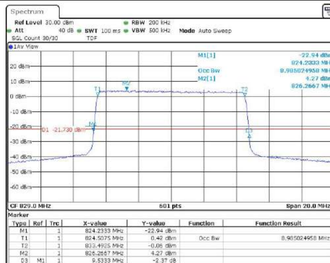
Band5-10MHz-QPSK-20525-50RB#0
