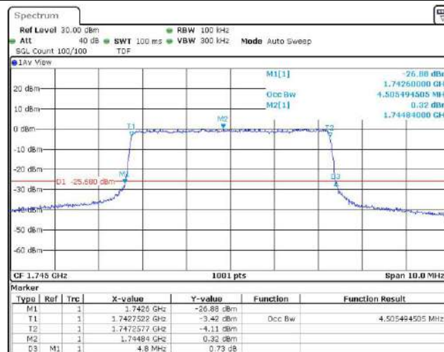
Band66-5MHz-QPSK-132647-25RB#0
