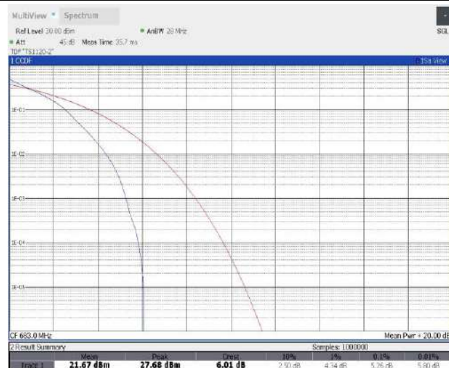
Band71-20MHz-QPSK-133322-100RB#0
