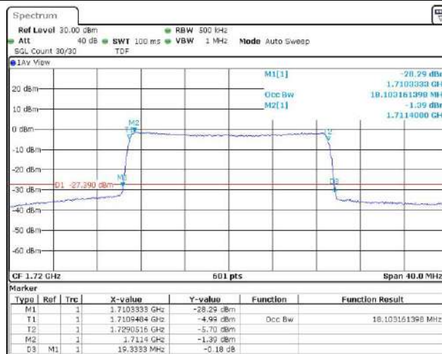
Band4-20MHz-16QAM-20175-100RB#0
