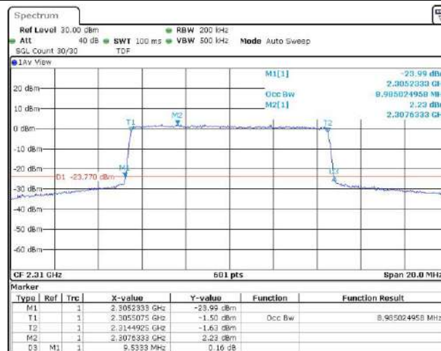
Band30-10MHz-16QAM-27710-50RB#0
