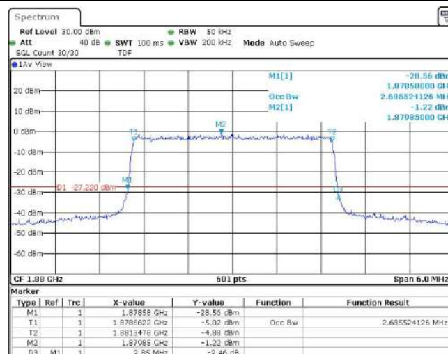
Band2-3MHz-16QAM-18900-15RB#0
