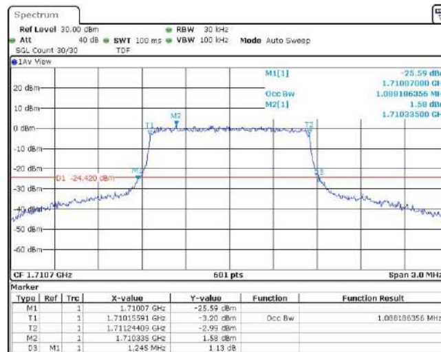
Band66-1.4MHz-16QAM-132322-6RB#0
