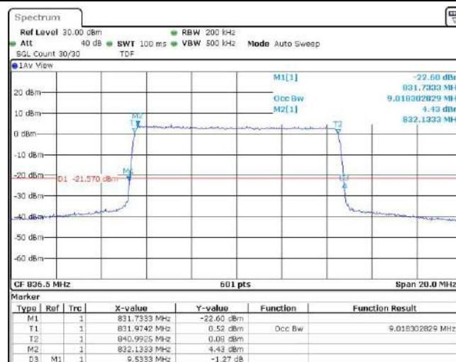
Band5-10MHz-QPSK-20600-50RB#0
