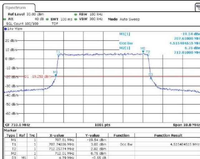
Band17-5MHz-16QAM-23825-25RB#0
