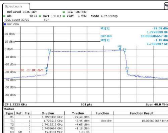
Band4-20MHz-16QAM-20300-100RB#0
