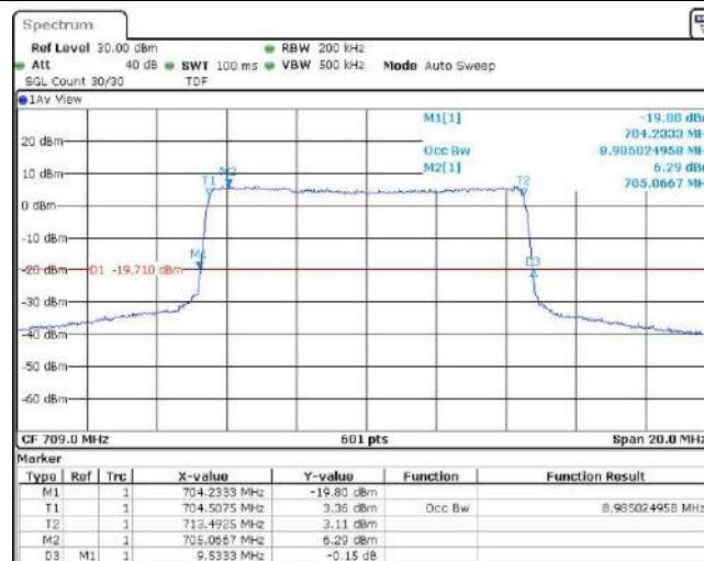
Band17-10MHz-QPSK-23790-50RB#0
