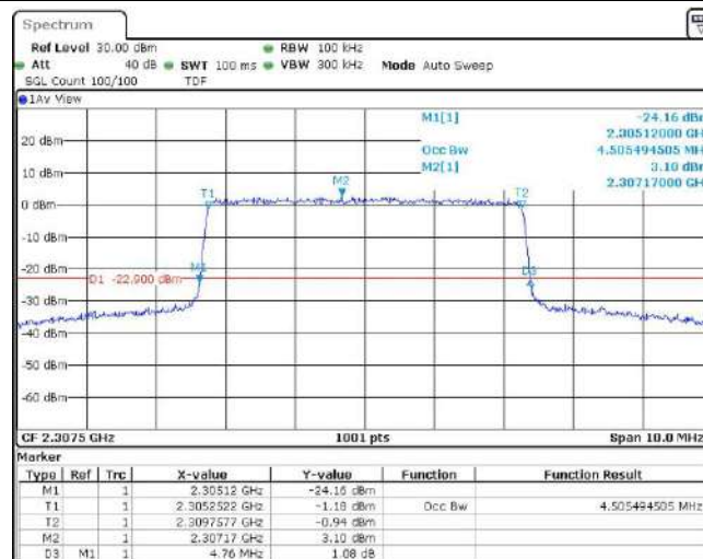
Band30-5MHz-16QAM-27710-25RB#0
