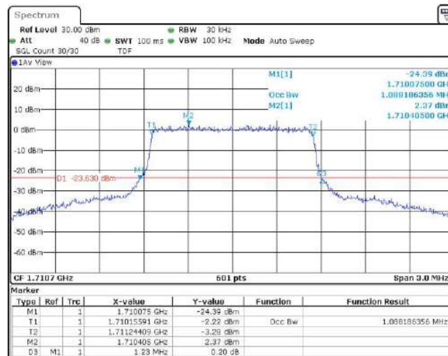
Band66-1.4MHz-QPSK-132322-6RB#0
