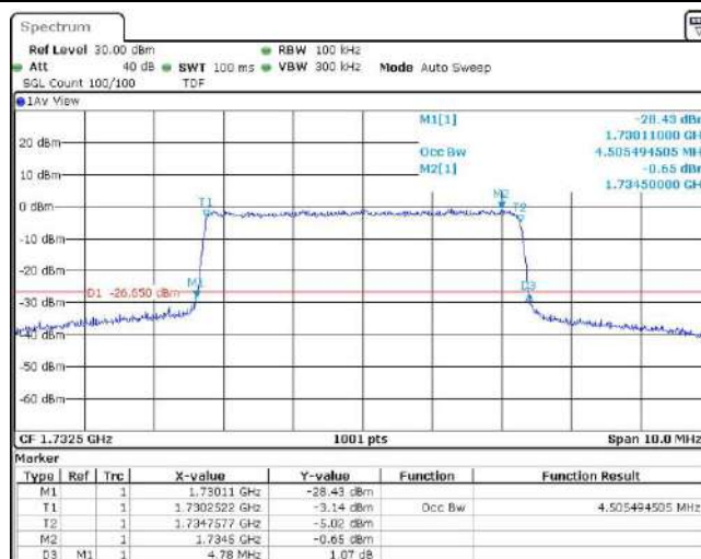
Band4-5MHz-16QAM-20375-25RB#0
