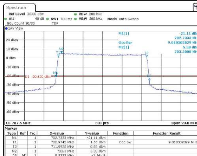
Band12-10MHz-16QAM-23130-50RB#0
