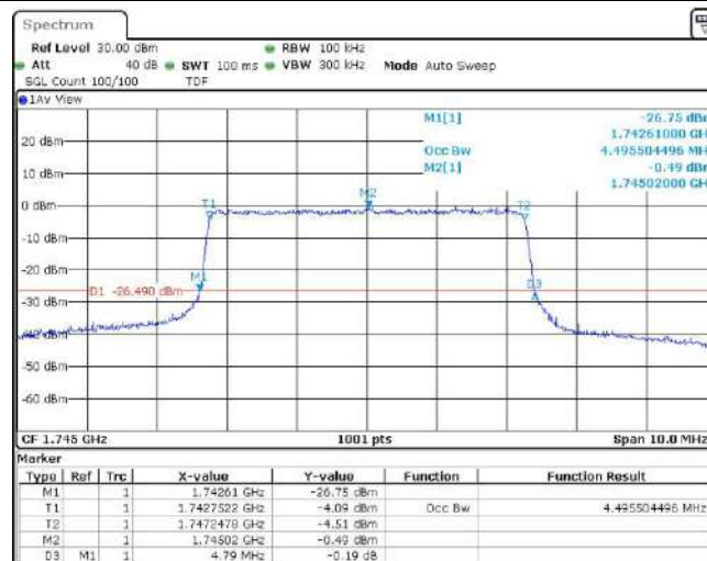
Band66-5MHz-16QAM-132647-25RB#0
