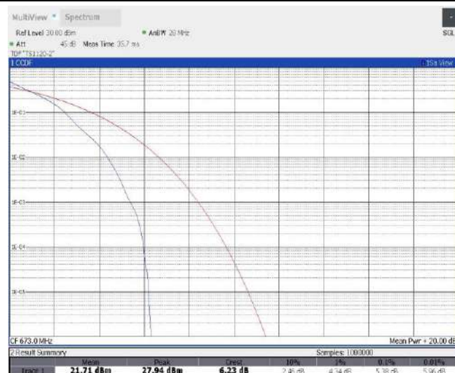
Band71-20MHz-QPSK-133222-100RB#0
