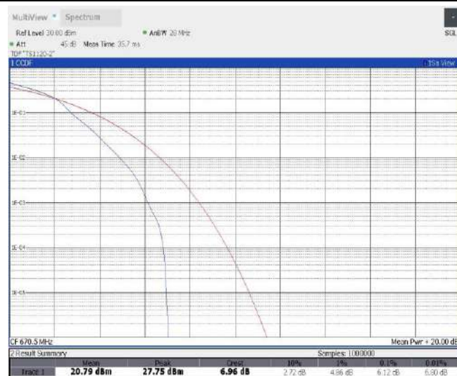
Band71-15MHz-16QAM-133197-75RB#0
