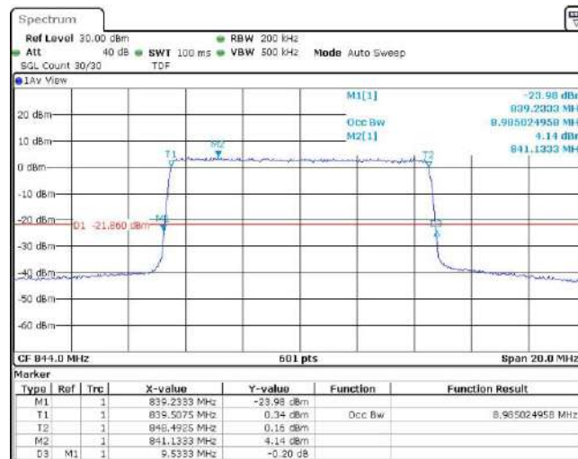
Band5-10MHz-16QAM-20450-50RB#0
