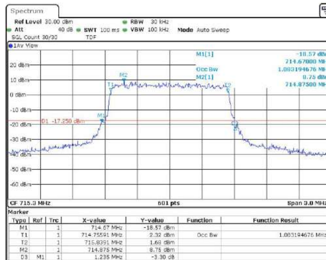
Band12-1.4MHz-16QAM-23017-6RB#0
