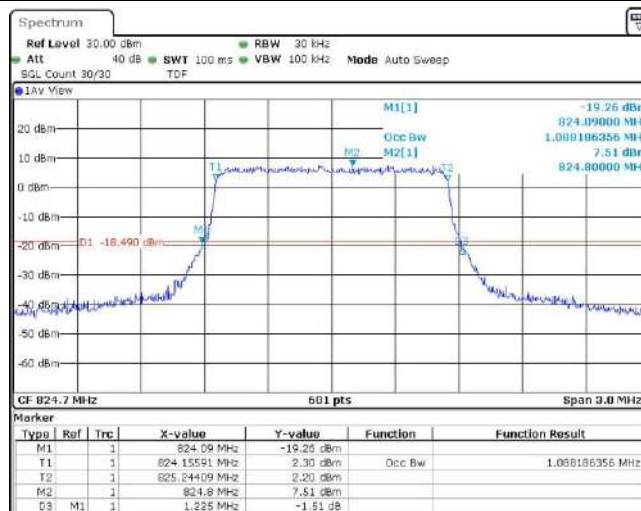
Band5-1.4MHz-QPSK-20525-6RB#0
