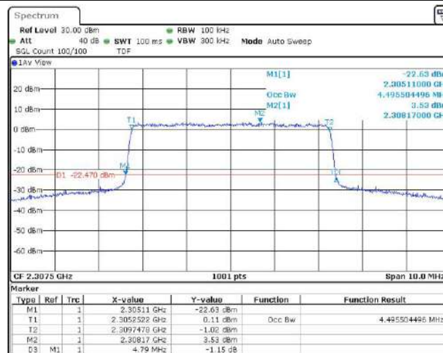
Band30-5MHz-QPSK-27710-25RB#0
