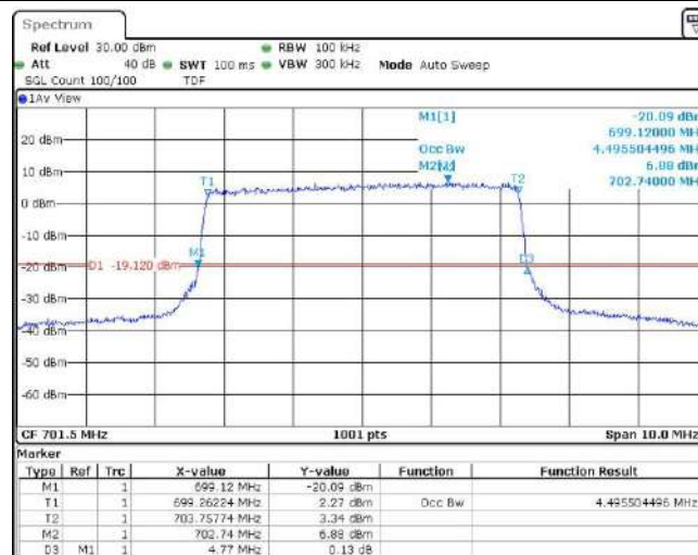
Band12-5MHz-16QAM-23095-25RB#0
