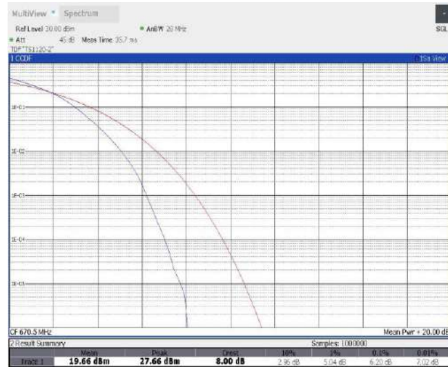
Band71-15MHz-16QAM-133297-1RB#0
