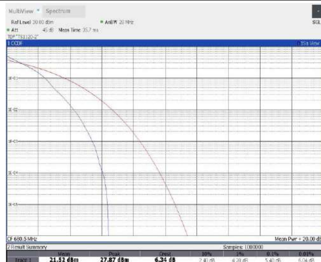
Band71-15MHz-QPSK-133297-75RB#0
