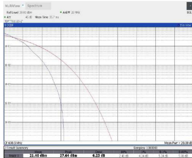
Band71-15MHz-QPSK-133397-75RB#0
