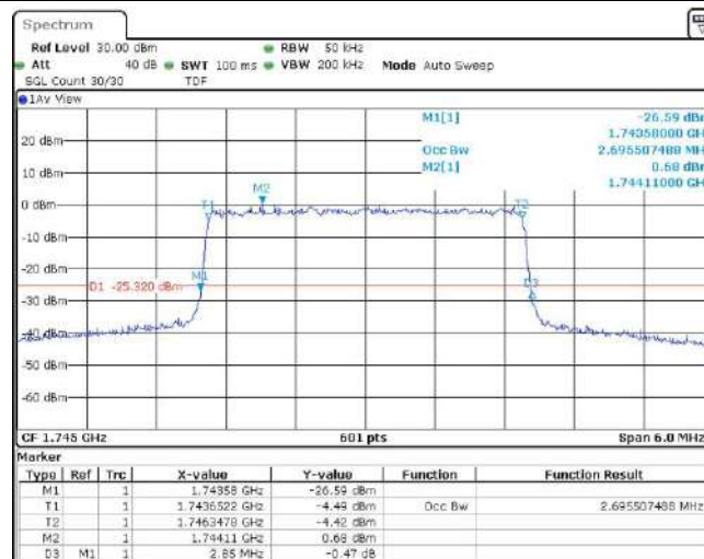
Band66-3MHz-QPSK-132657-15RB#0
