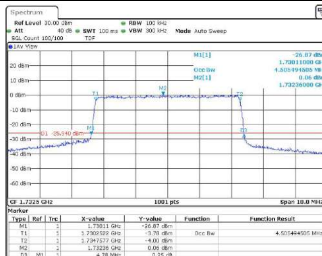
Band4-5MHz-QPSK-20175-25RB#0
