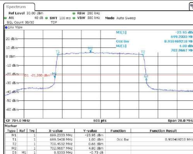
Band12-10MHz-16QAM-23095-50RB#0
