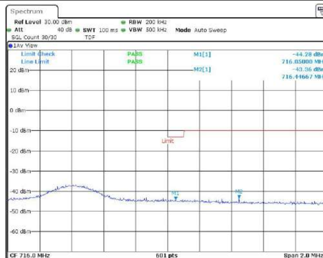
Band12-10MHz-16QAM-23130-1RB#49
