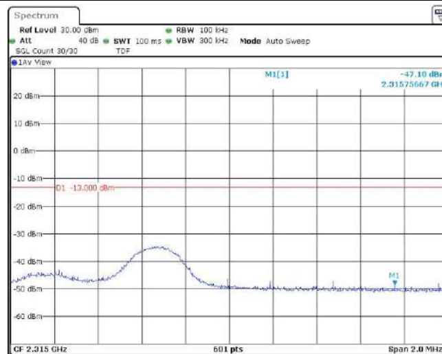
Band30-5MHz-QPSK-27735-1RB#24
