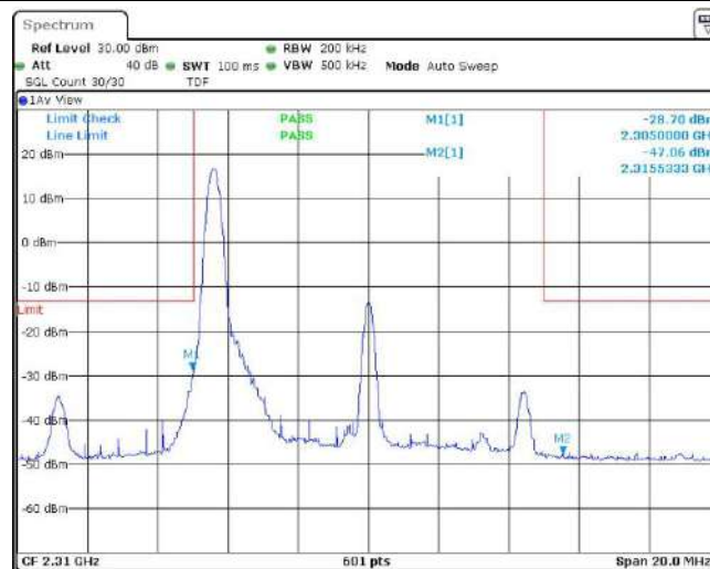
Band30-10MHz-QPSK-27710-1RB#49
