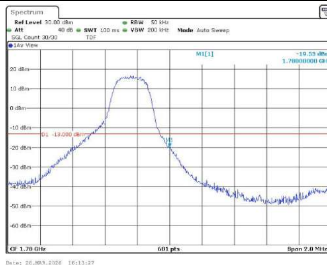
Band66-3MHz-QPSK-132657-15RB#0
