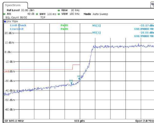
Band12-1.4MHz-16QAM-23173-1RB#0
