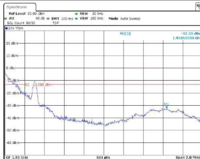
Band2-1.4MHz-QPSK-19193-1RB#5
