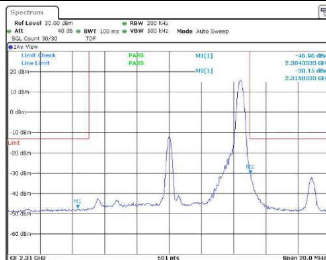
Band30-10MHz-16QAM-27710-50RB#0
