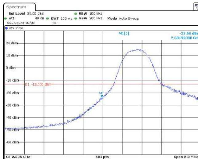
Band30-5MHz-16QAM-27685-1RB#24
