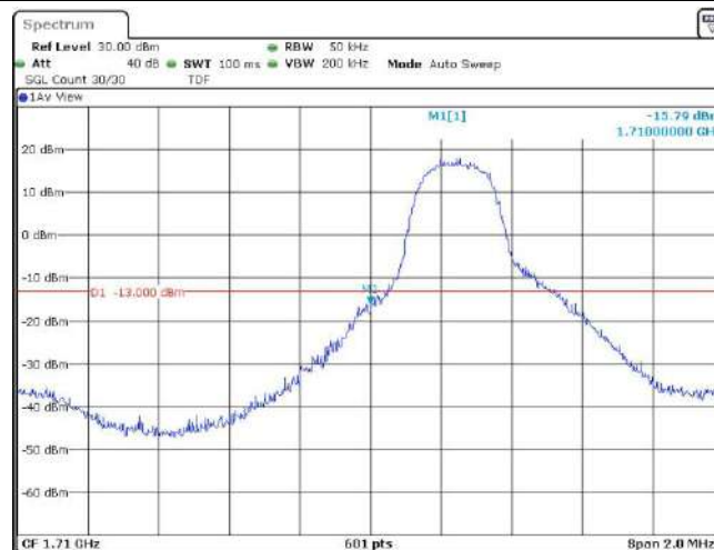
Band66-3MHz-QPSK-131987-1RB#0
