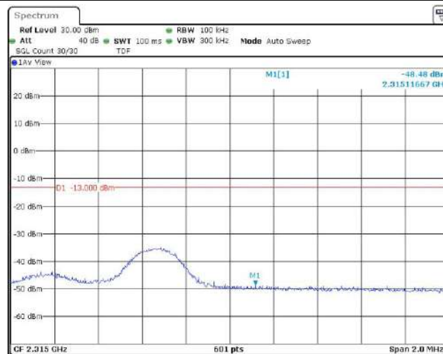
Band30-5MHz-16QAM-27735-1RB#24
