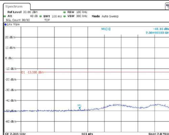
Band30-5MHz-QPSK-27685-25RB#0
