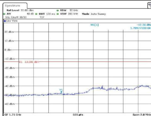
Band66-3MHz-QPSK-131987-1RB#14
