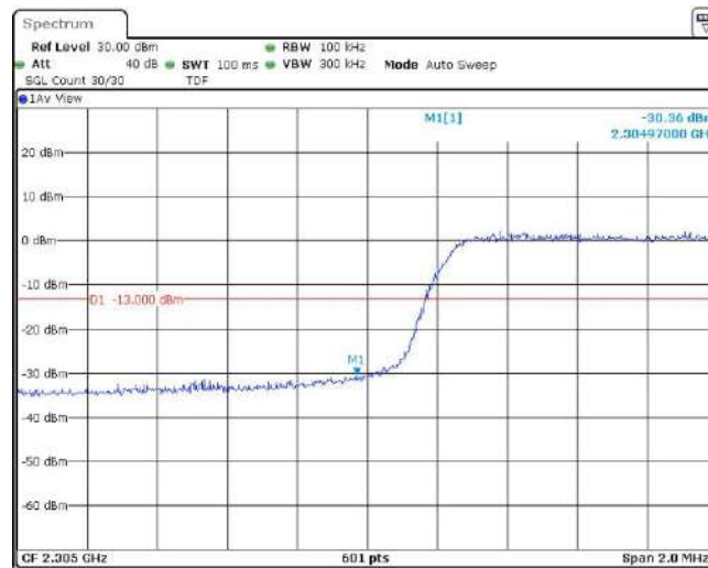
Band30-5MHz-QPSK-27735-1RB#0
