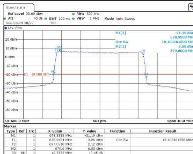
Band71-20MHz-16QAM-133222-100RB#0
