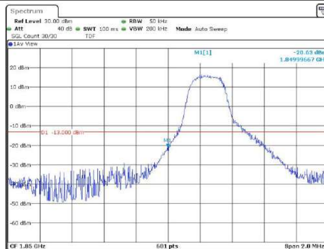
Band2-3MHz-16QAM-18615-1RB#0
