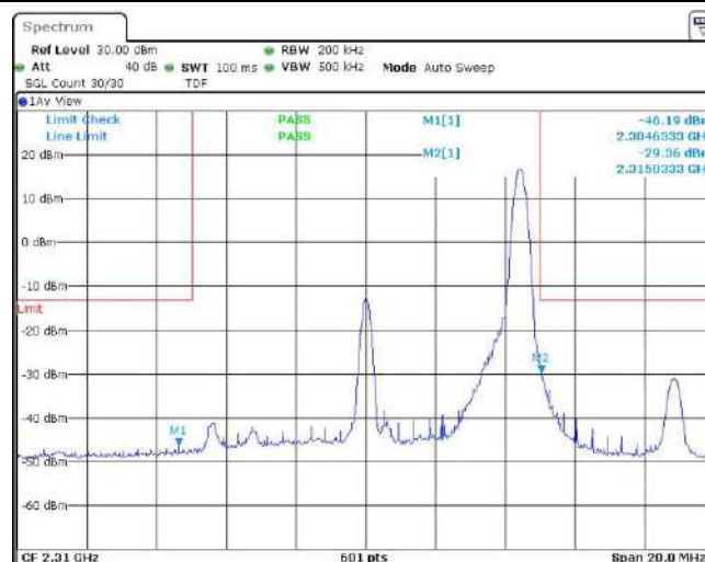
Band30-10MHz-QPSK-27710-50RB#0
