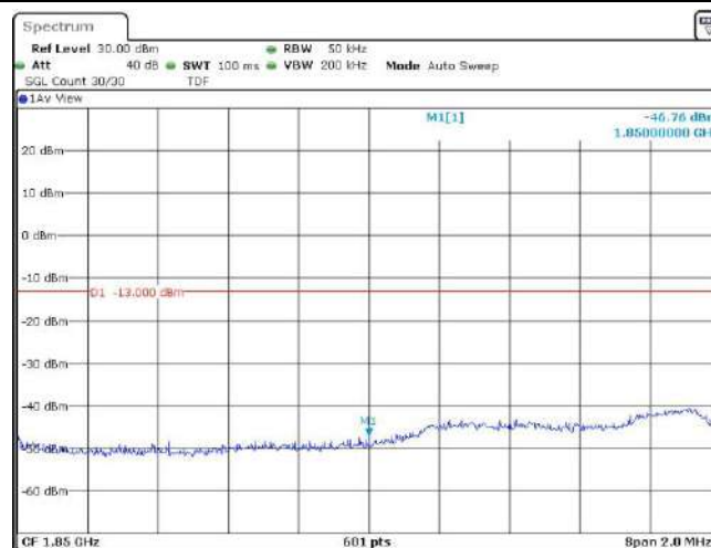
Band2-3MHz-16QAM-18615-1RB#14
