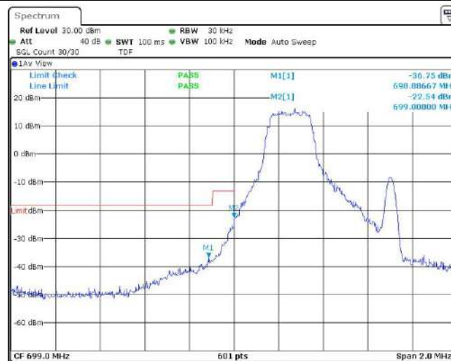
Band12-1.4MHz-16QAM-23017-1RB#5
