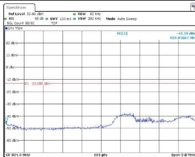
Band5-3MHz-QPSK-20415-15RB#0
