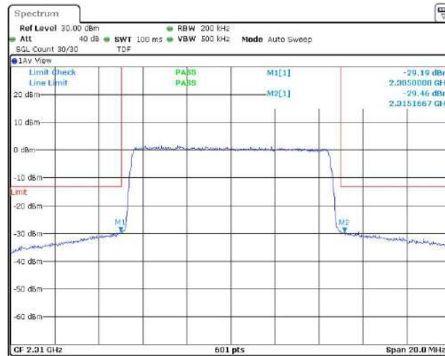
Band30-10MHz-16QAM-27710-1RB#0
