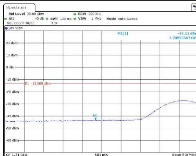
Band66-15MHz-QPSK-132047-75RB#0
