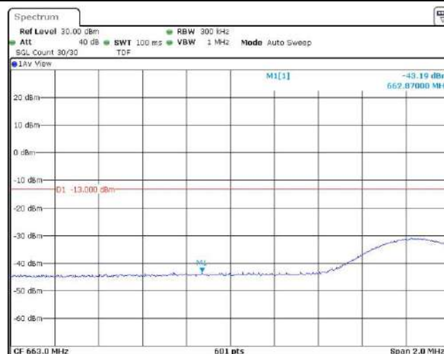
Band71-15MHz-QPSK-133197-75RB#0
