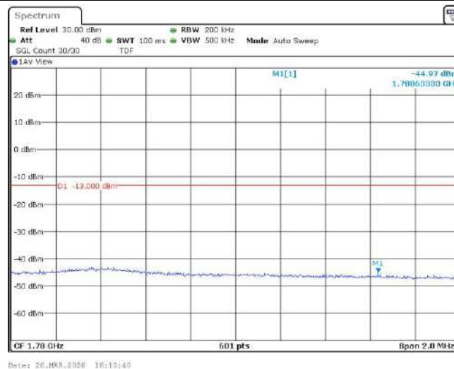
Band66-10MHz-QPSK-132622-1RB#49
