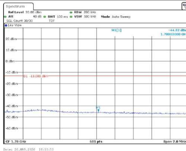
Band66-10MHz-16QAM-132622-1RB#49
