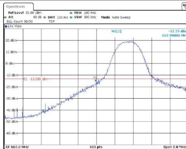
Band71-5MHz-16QAM-133147-1RB#24
