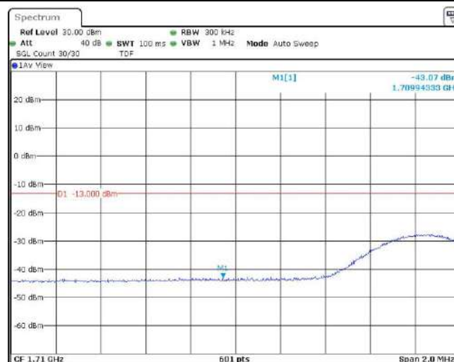
Band66-15MHz-16QAM-132047-75RB#0
