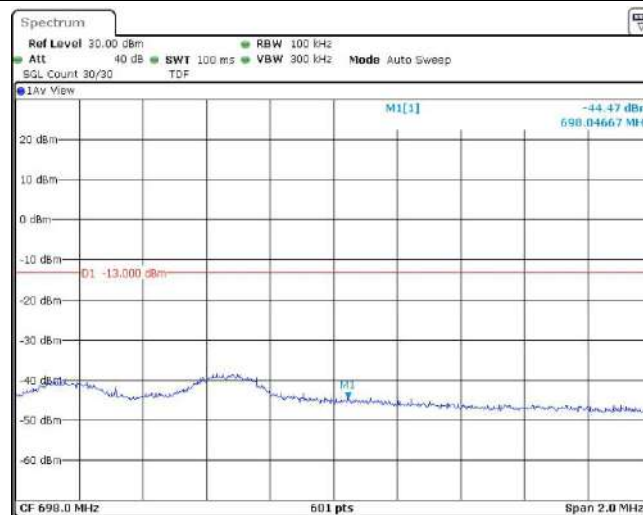
Band71-5MHz-QPSK-133447-1RB#24
