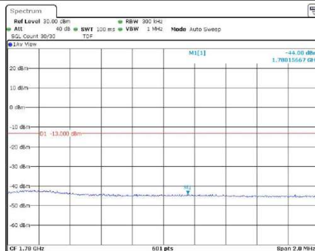
Band66-15MHz-16QAM-132597-1RB#74
