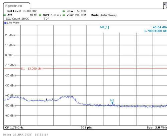
Band66-3MHz-16QAM-132657-1RB#14
