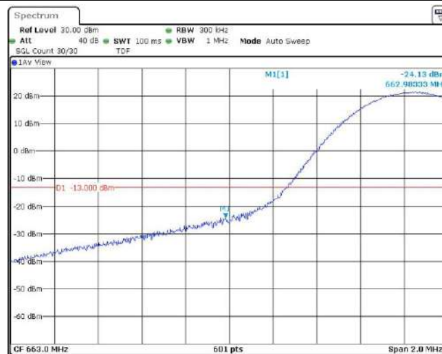
Band71-15MHz-QPSK-133197-1RB#74
