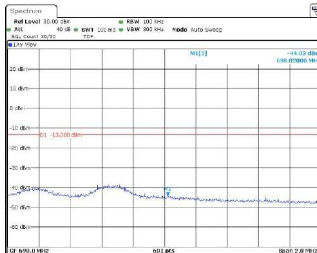
Band71-5MHz-16QAM-133447-1RB#24
