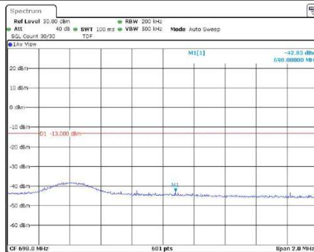
Band71-10MHz-16QAM-133422-1RB#49
