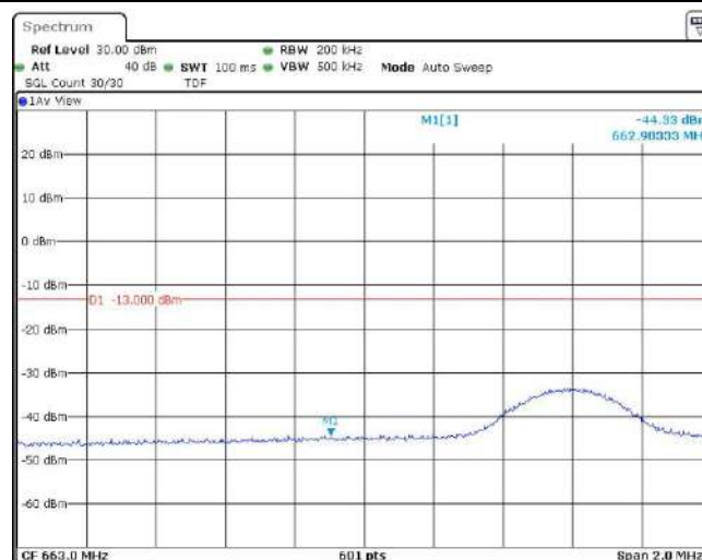
Band71-10MHz-16QAM-133172-50RB#0
