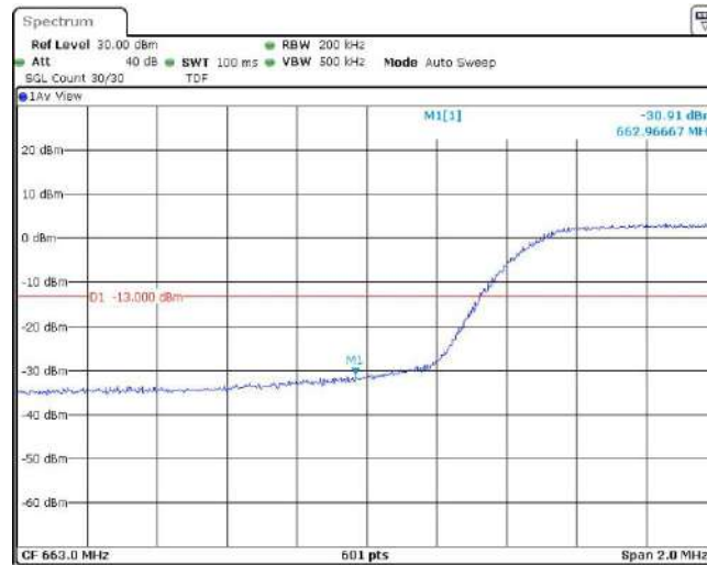
Band71-10MHz-16QAM-133422-1RB#0
