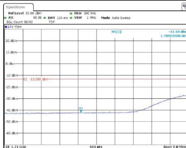
Band66-20MHz-QPSK-132072-100RB#0
