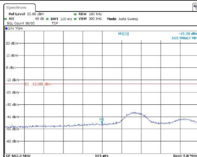
Band71-5MHz-16QAM-133147-25RB#0
