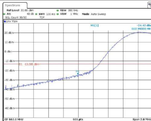
Band71-15MHz-16QAM-133197-1RB#74
