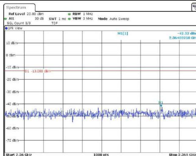
Band30-5MHz-16QAM-27735-1RB#0-Range13:2365~26500MHz
