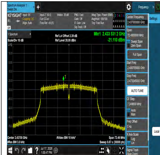
11n40SISO-Ant1-2437-PASS
