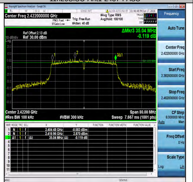
11n40SISO-Ant1-2422-PASS
