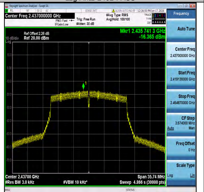
11n20SISO-Ant1-2437-PASS
