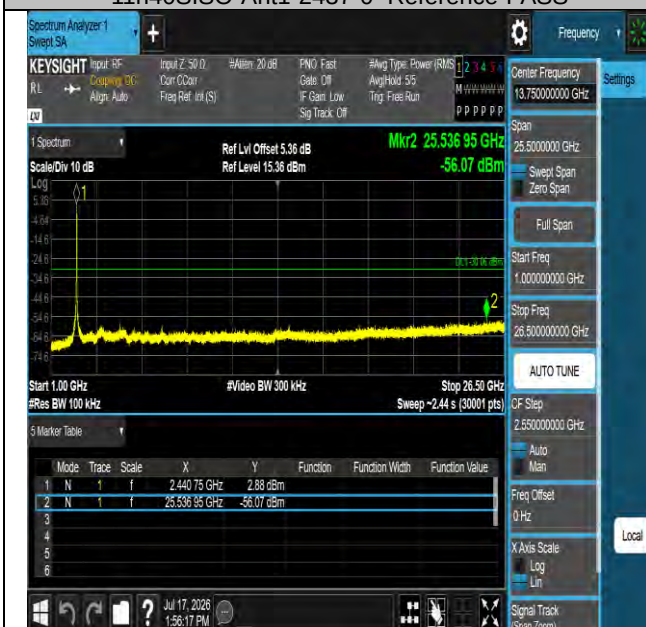
11n40SISO-Ant1-2437-1000~26500-PASS
