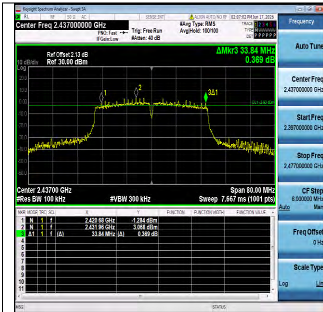
11n40SISO-Ant1-2437-PASS
