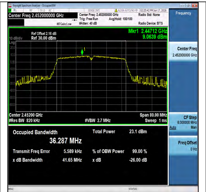
11n40SISO-Ant1-2452
