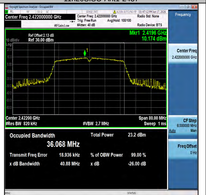
11n40SISO-Ant1-2422
