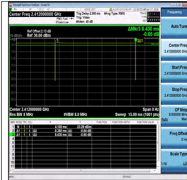
NTNV-11b-Ant1-2412
