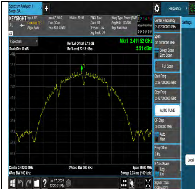
11b-Ant1-2412-0~Reference-PASS
