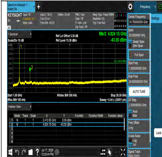
11b-Ant1-2412-1000~26500-PASS
