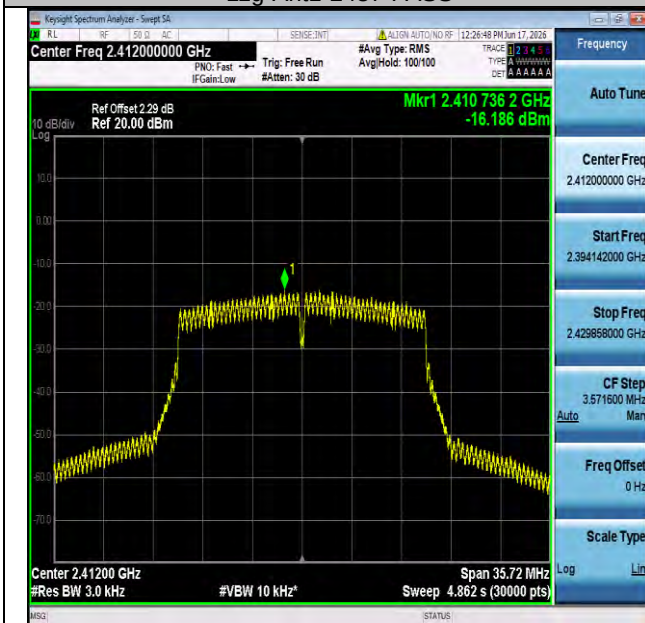
11n20SISO-Ant1-2412-PASS
