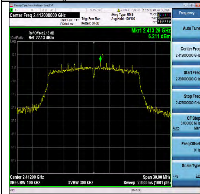
11n20SISO-Ant1-2412-0~Reference-PASS
