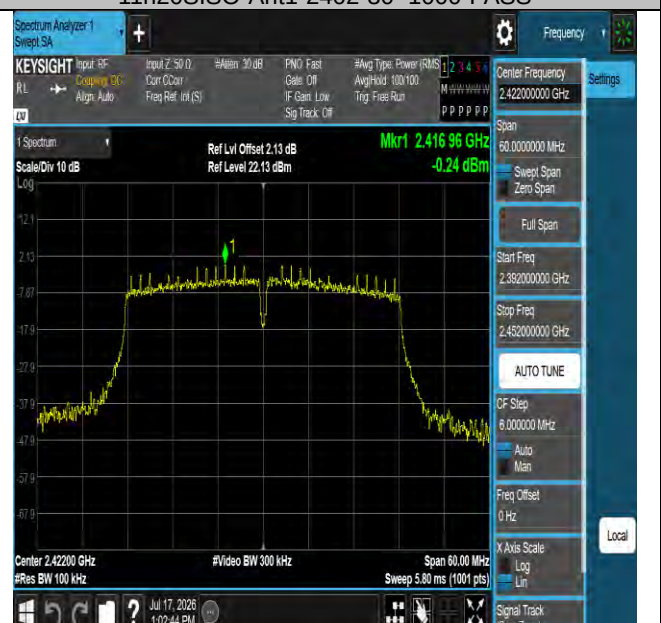
11n40SISO-Ant1-2422-0~Reference-PASS
