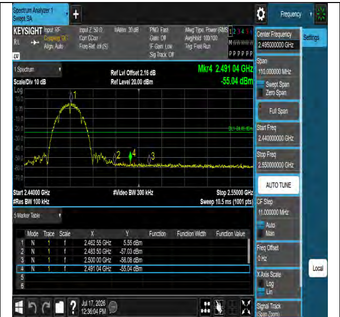
11b-Ant1-2462-PASS
