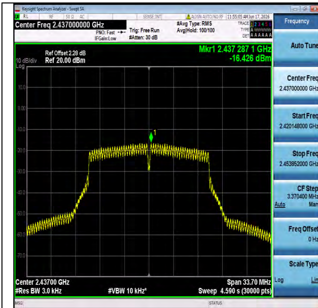
11g-Ant1-2437-PASS
