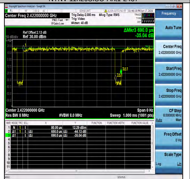
NTNV-11n40SISO-Ant1-2422
