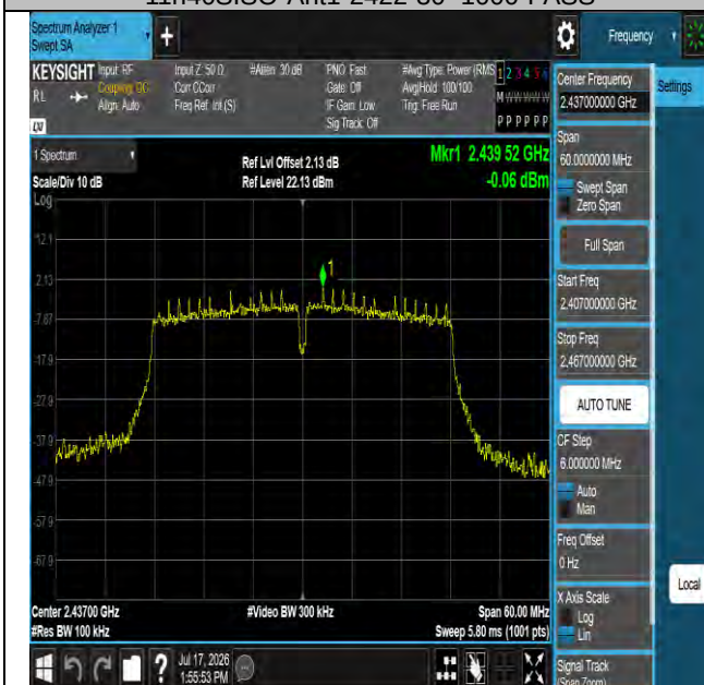
11n40SISO-Ant1-2437-0~Reference-PASS
