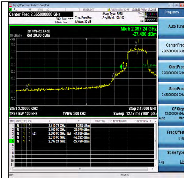
11n20SISO-Ant1-2412-PASS
