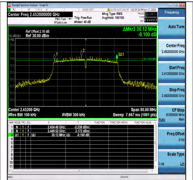
11n40SISO-Ant1-2452-PASS
