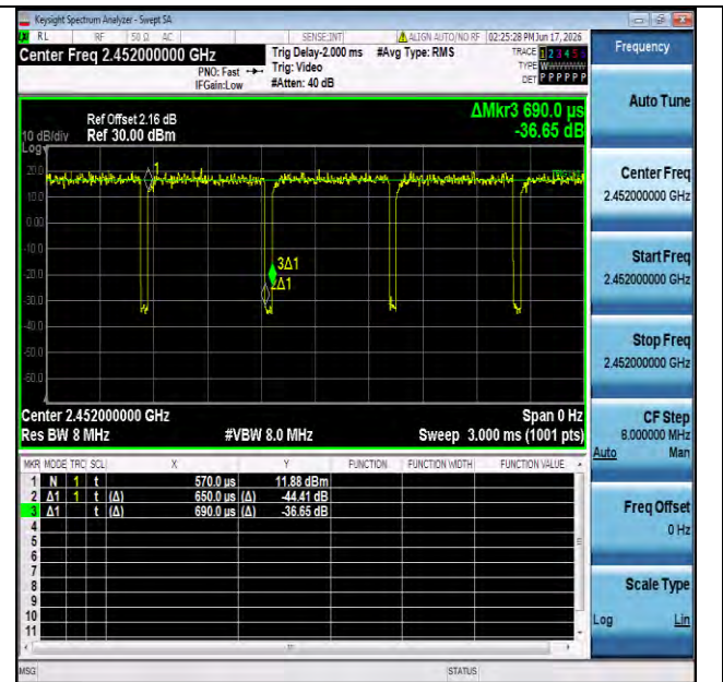
NTNV-11n40SISO-Ant1-2452
