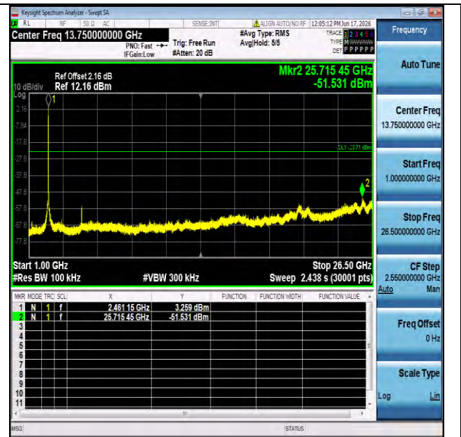
11g-Ant1-2462-1000~26500-PASS
