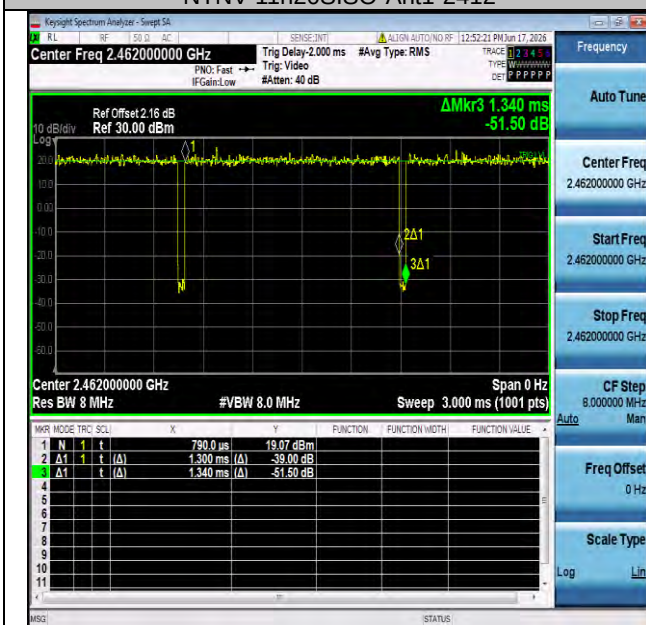
NTNV-11n20SISO-Ant1-2462
