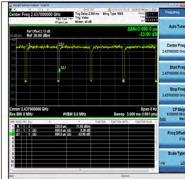
NTNV-11n40SISO-Ant1-2437
