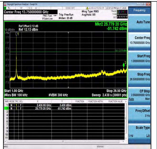
11n20SISO-Ant1-2437-1000~26500-PASS
