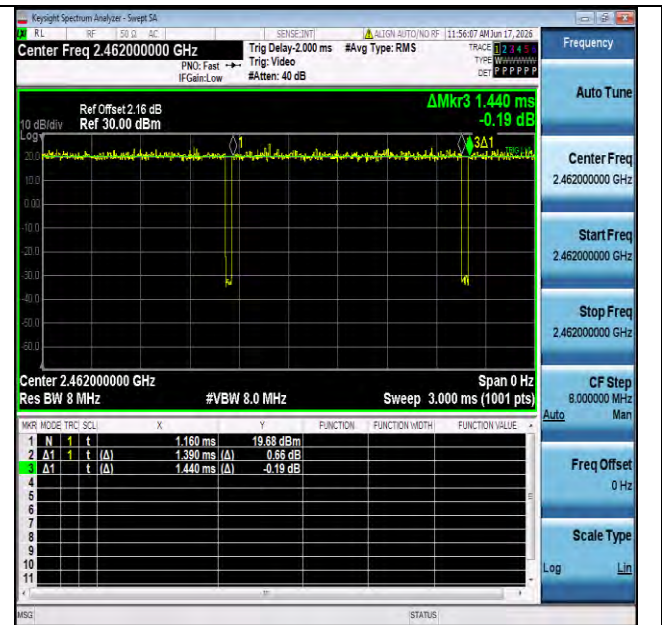
NTNV-11g-Ant1-2462
