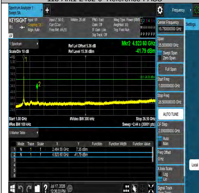
11b-Ant1-2462-1000~26500-PASS
