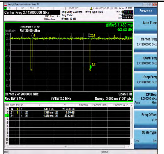
NTNV-11g-Ant1-2412
