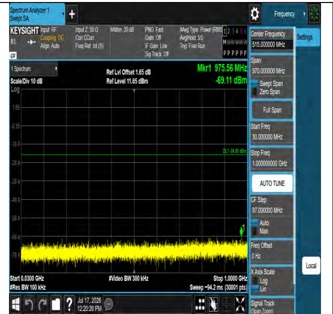
11b-Ant1-2412-30~1000-PASS
