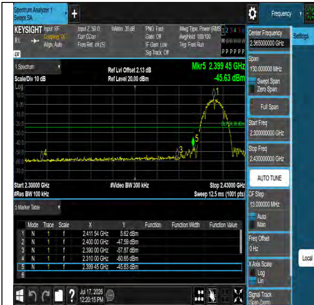
11b-Ant1-2412-PASS
