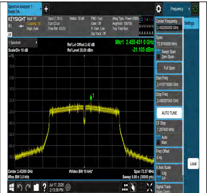
11n40SISO-Ant1-2452-PASS
