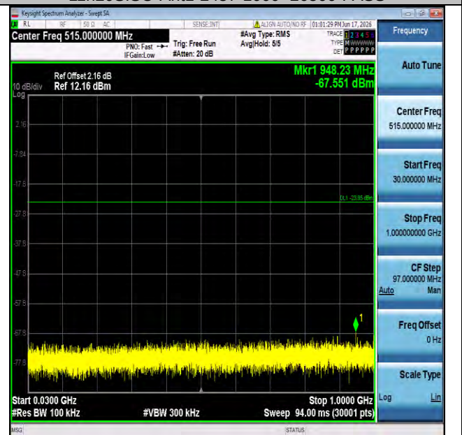
11n20SISO-Ant1-2462-30~1000-PASS
