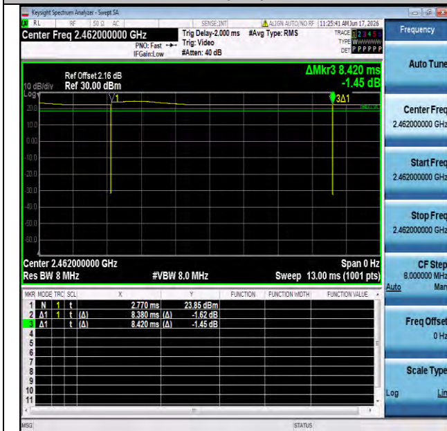
NTNV-11b-Ant1-2462
