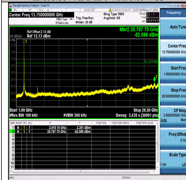
11n20SISO-Ant1-2412-1000~26500-PASS
