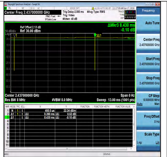
NTNV-11b-Ant1-2437
