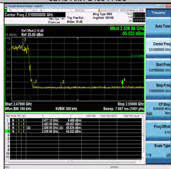
3D5H-Ant1-Hop 2480-PASS
