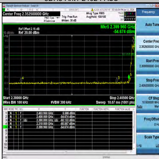
3D5H-Ant1-Hop 2402-PASS
