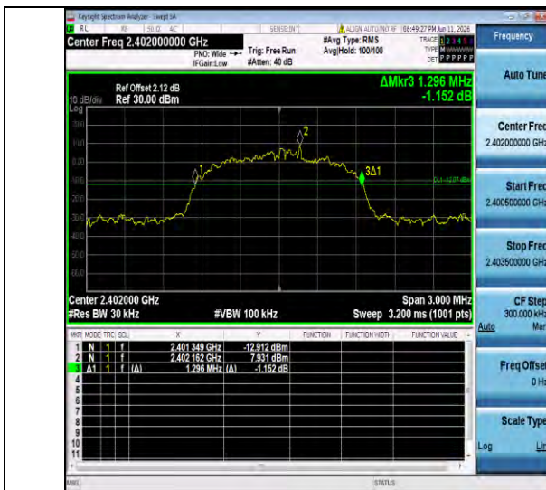
3DH5-Ant1-2402
