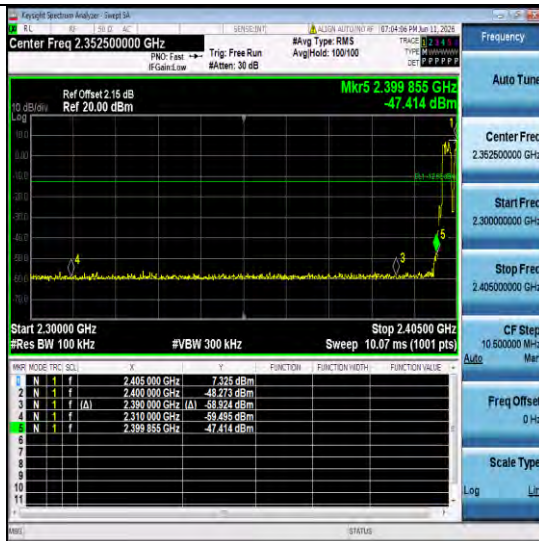
2D5H-Ant1-Hop 2402-PASS
