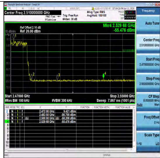
2D5H-Ant1-Hop 2480-PASS
