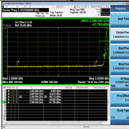
3D5H-Ant1-2402-PASS
