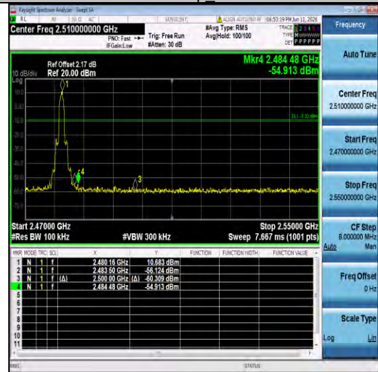
3D5H-Ant1-2480-PASS
