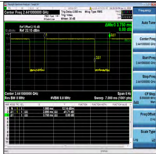
NTNV-3DH5-Ant1-2441
