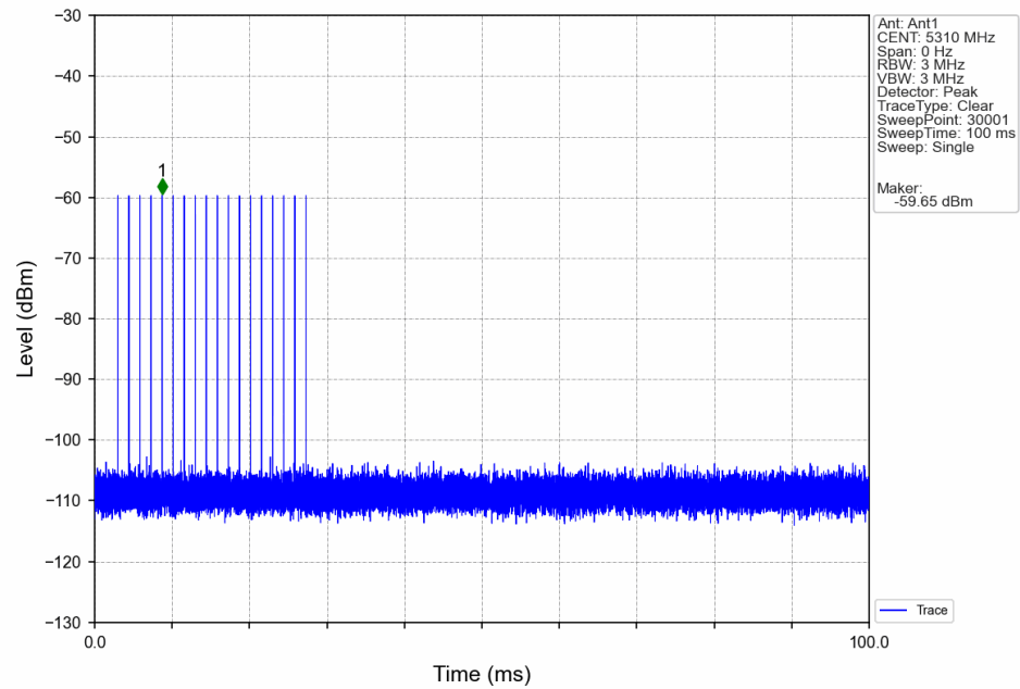
Radar Signal 5310
