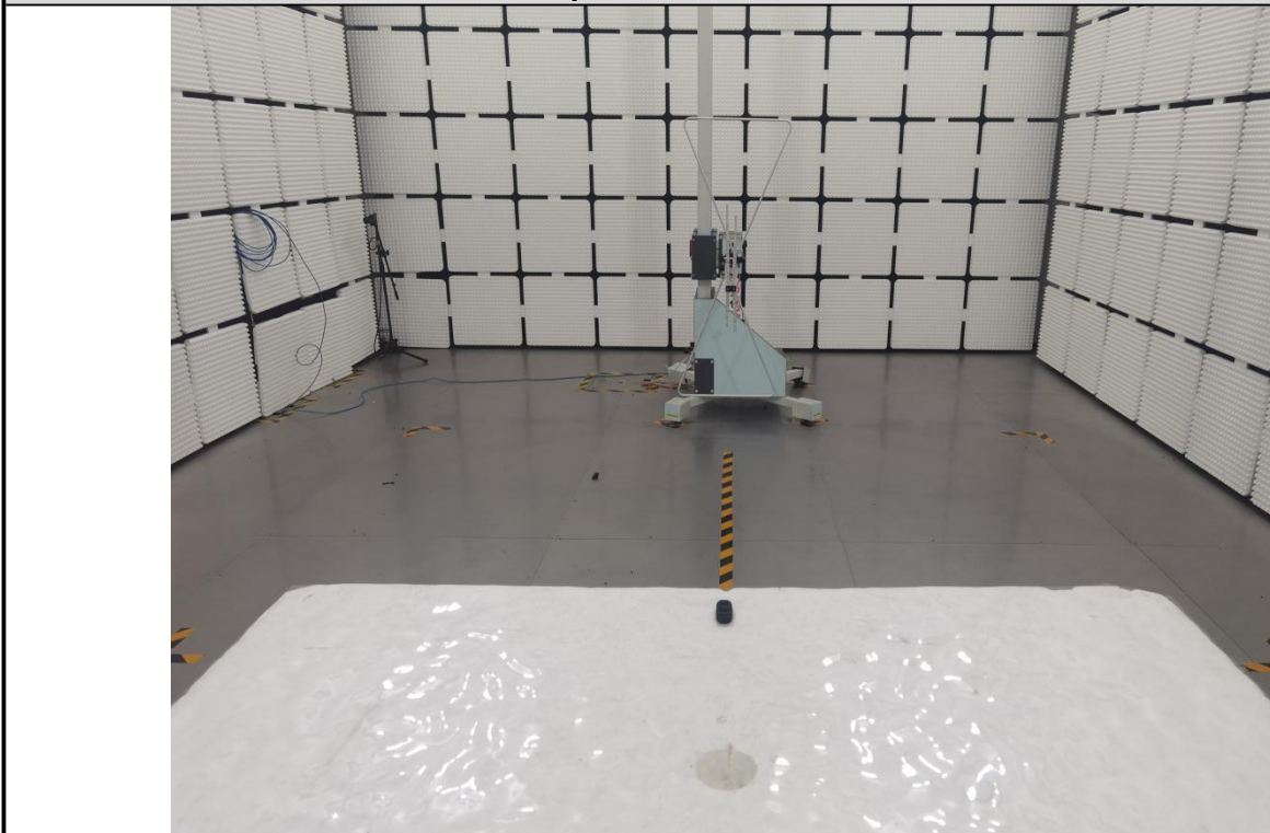
Radiated Spurious Emission, Below 1GHz
