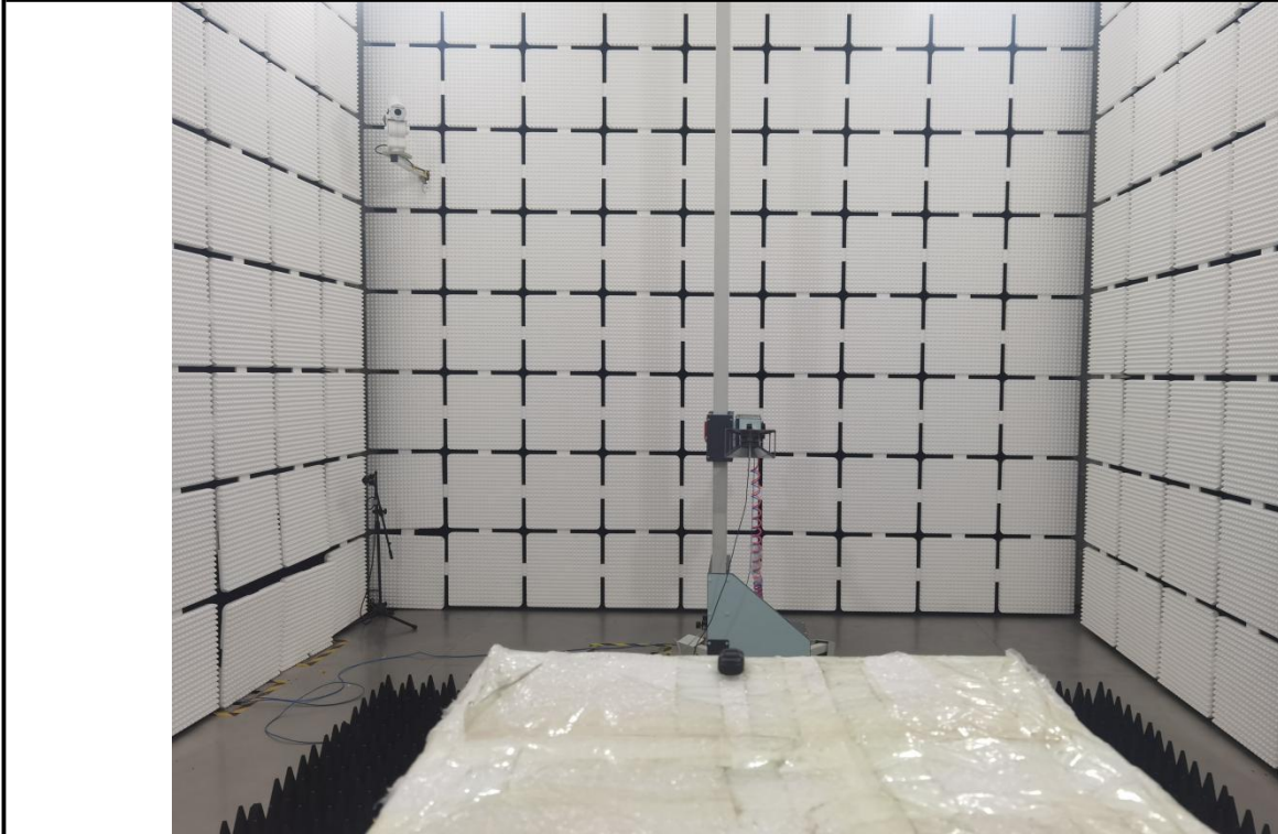
Radiated Spurious Emission, Above 1GHz
