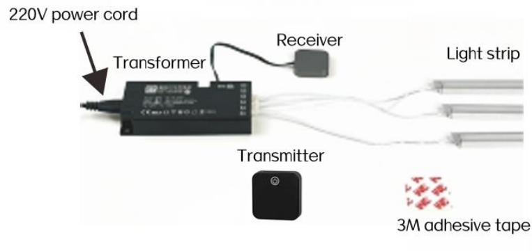
Operation installation wiring diagram
