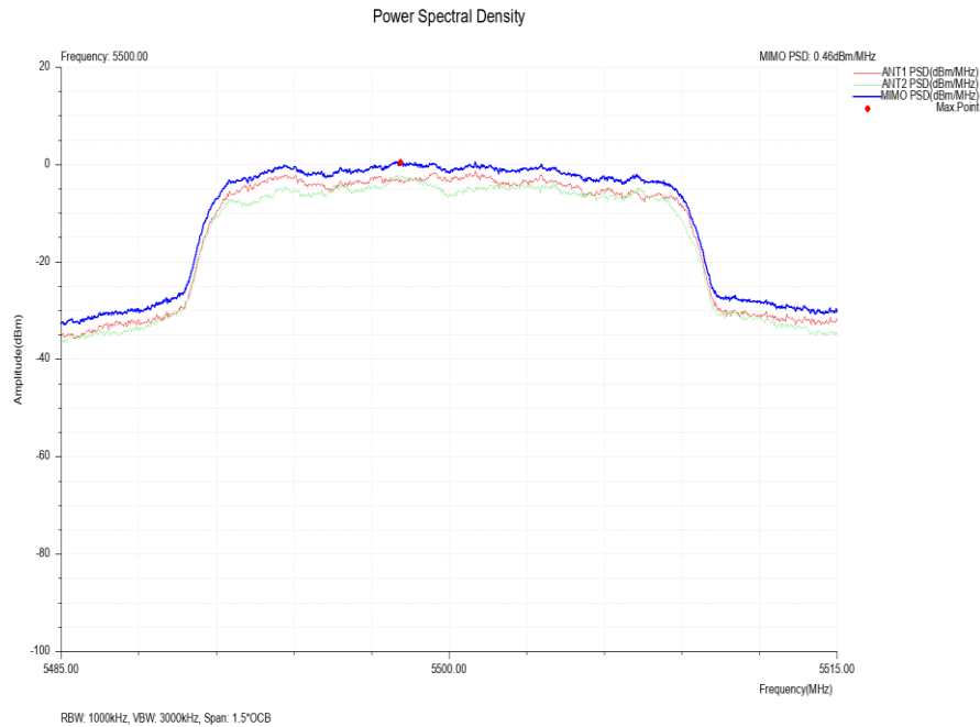
NVNT MIMO TX 802_11n(HT20) Power Spectral Density 5500
