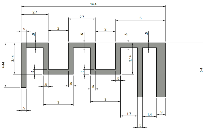
Antenna Dimensions
