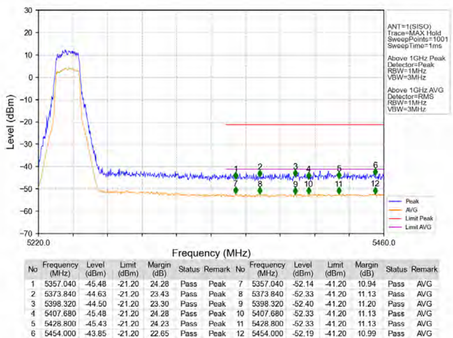
802.11a_HCH_5240MHz_Ant1_NTNV
