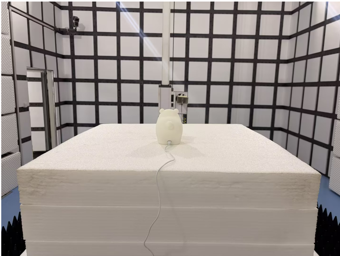
Radiated Emission - Front View (18GHz - 40GHz)
