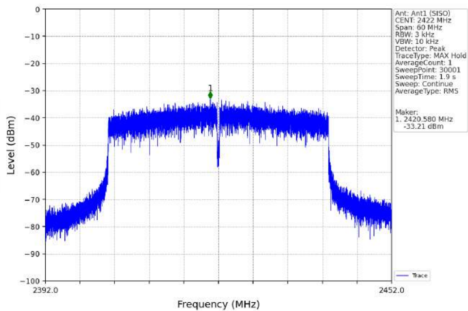
802.11ax(HEW40)_LCH_2422MHz_SU_/_Ant1 (SISO)_NTNV
