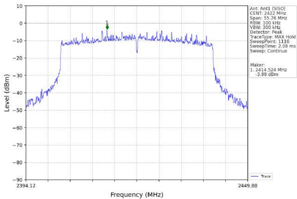
802.11ax(HEW40)_LCH_2422MHz_SU_/_Ant1 (SISO)_NTNV
