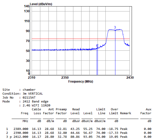
11n_HT(20M)_TX_CH_01_Vertical-Peak
