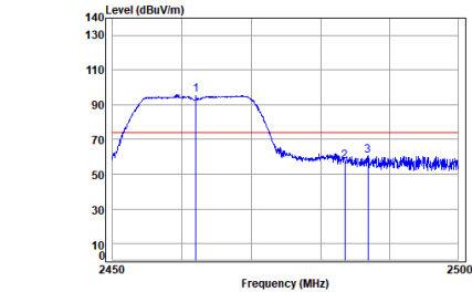
11g_TX_CH_11_Horizontal-Peak
