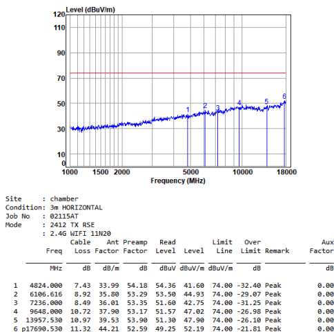
11n_HT(20M)_TX_CH_01_Horizontal-Peak
