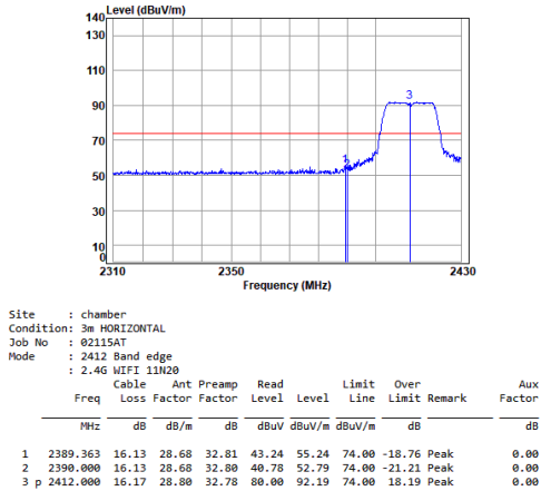
11n_HT(20M)_TX_CH_01_Horizontal-Peak
