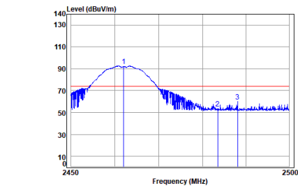
11b_TX_CH_11_Vertical-Peak
