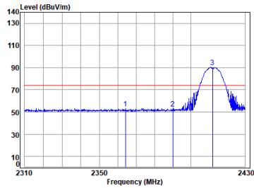
11b_TX_CH_01_Horizontal-Peak
