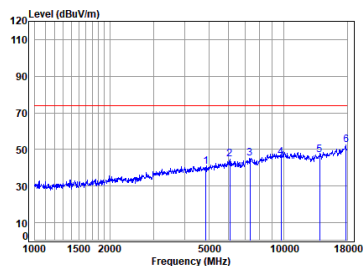
11n_HT(20M)_TX_CH_06_Horizontal-Peak
