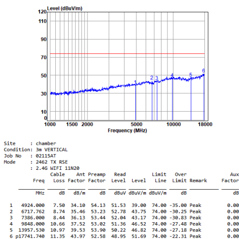
11n_HT(20M)_TX_CH_11_Vertical-Peak
