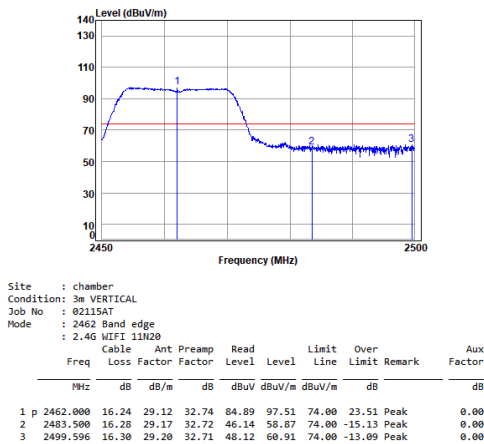
11n_HT(20M)_TX_CH_11_Vertical-Peak
