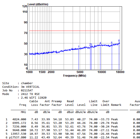
11n_HT(20M)_TX_CH_01_Vertical-Peak
