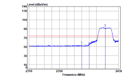
11g_TX_CH_01_Horizontal-Peak
