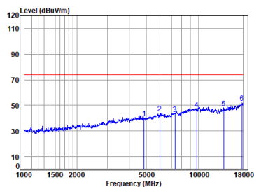
11n_HT(20M)_TX_CH_06_Vertical-Peak
