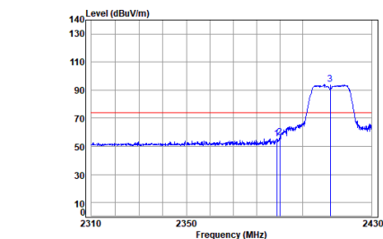
11g_TX_CH_01_Vertical-Peak
