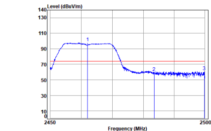
11g_TX_CH_11_Vertical-Peak
