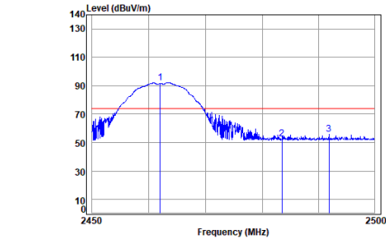
11b_TX_CH_11_Horizontal-Peak
