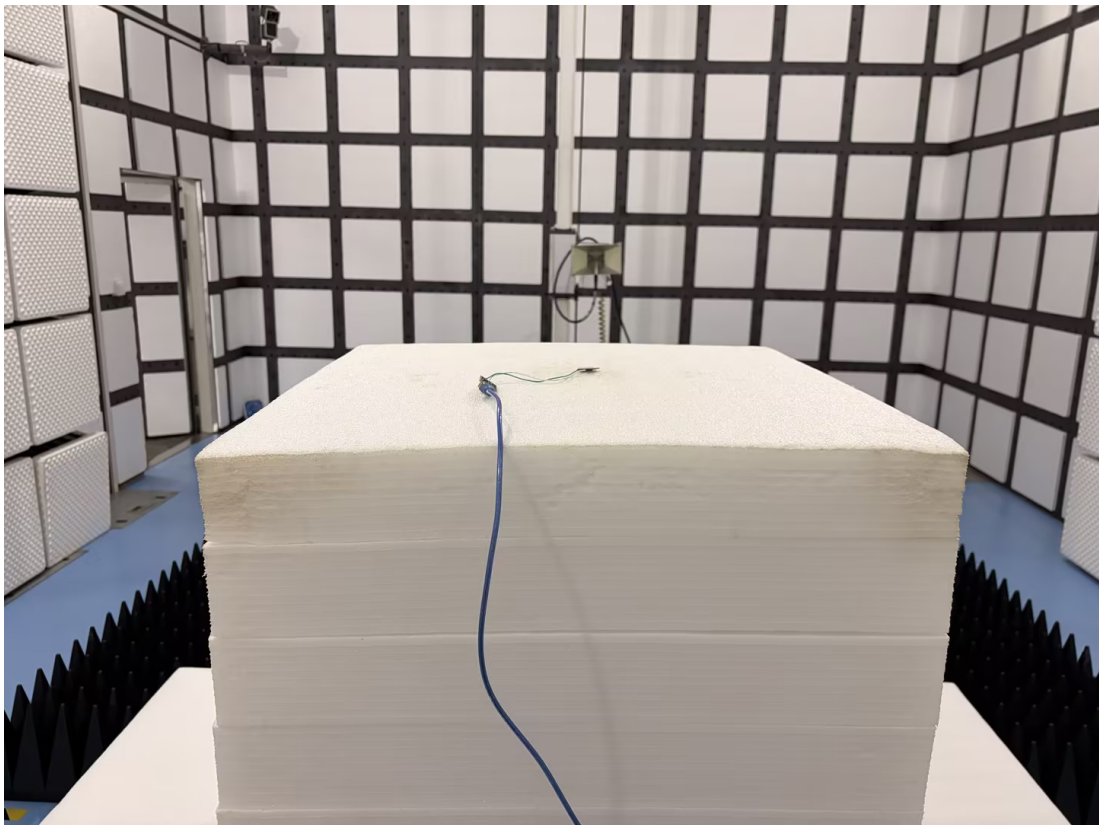
Radiated Emission - Front View (18GHz - 40GHz)
