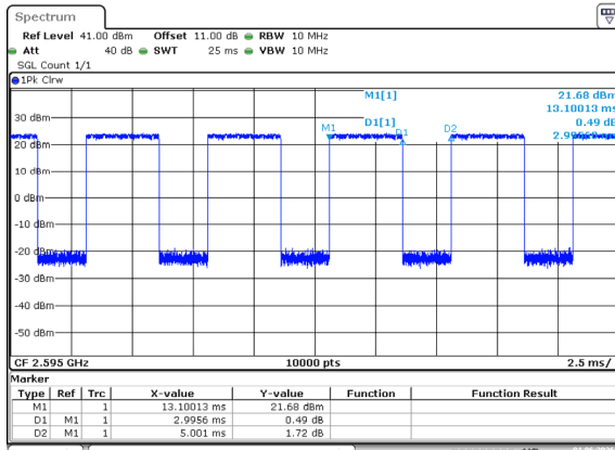
15MHz_Middle_QPSK_75@0
