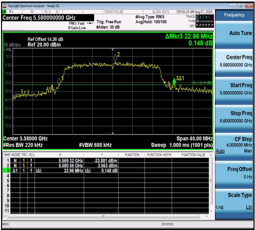
11AX20SISO-Ant1-5580
