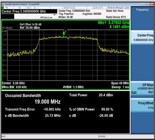
11AX20SISO-Ant1-5580
