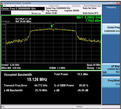
11AX20SISO-Ant1-5260
