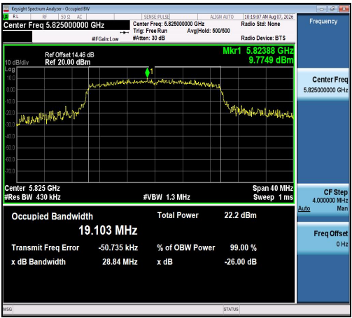
11AX20SISO-Ant1-5825
