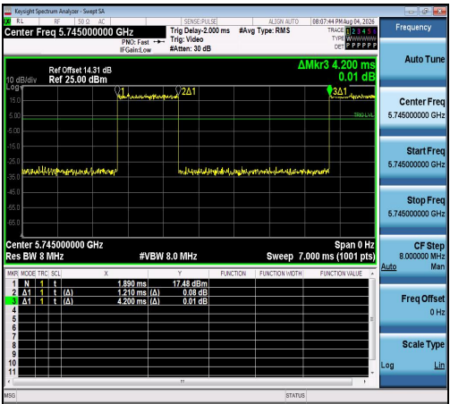
NTNV-11N20SISO-Ant1-5745
