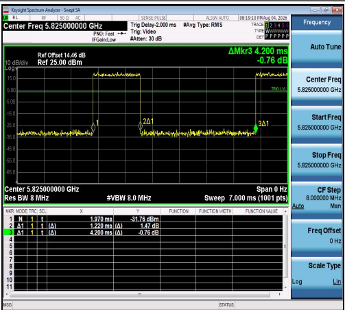
NTNV-11N20SISO-Ant1-5825
