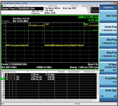
NTNV-11N20SISO-Ant1-5785
