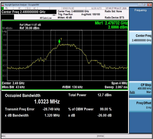
LE_1M-Ant1-2480
