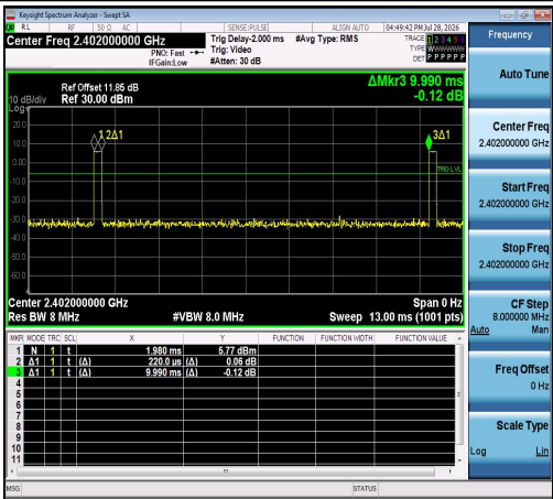
NTNV-LE_1M-Ant1-2402
