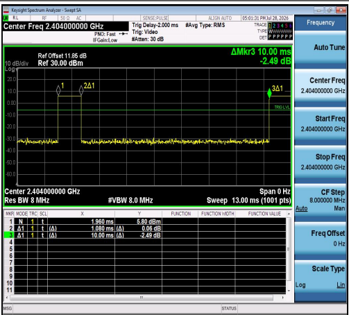
NTNV-LE_2M-Ant1-2404
