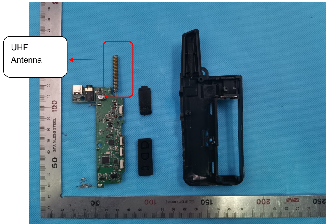
Internal View-2 of EUT
