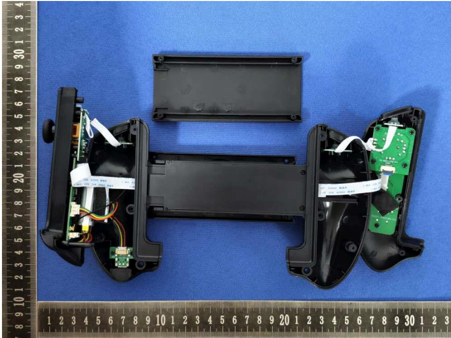
Model: BR-RC1-DM-BK EUT Internal View 1
