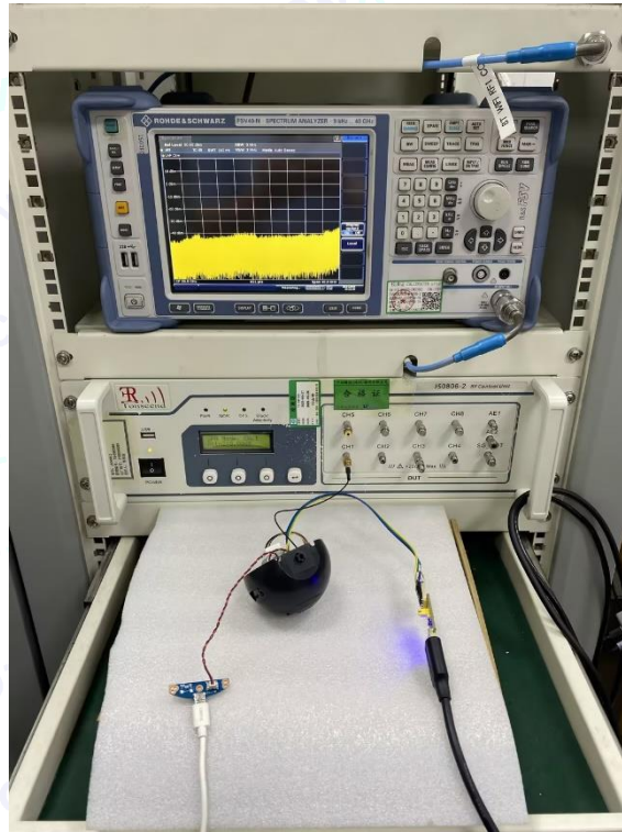
Photo of Setup for RF Conducted
