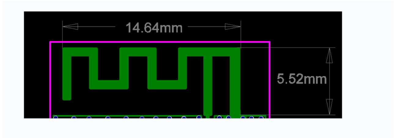
Picture 2 Antenna plots
