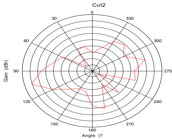
Vertical X-Z
