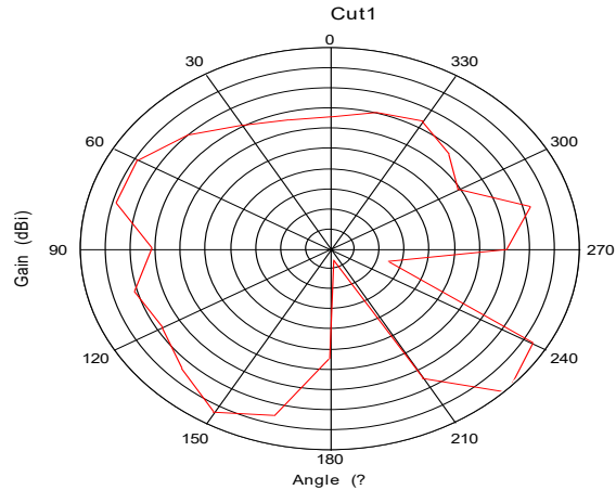
Vertical X-Y
