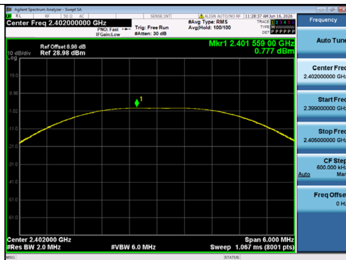
BLE_2M-Ant1-2402-PASS
