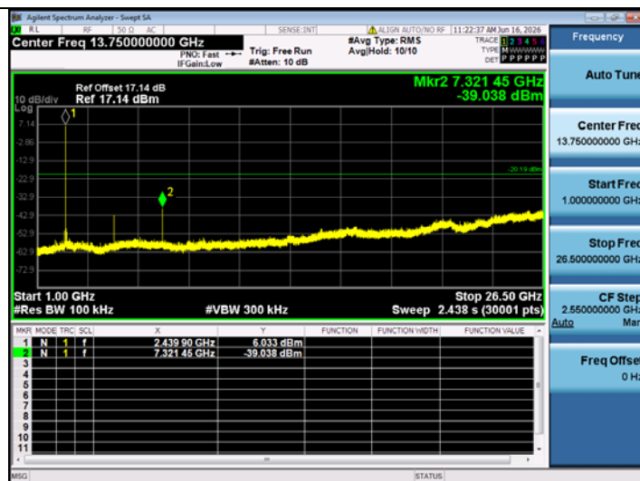
BLE_2M-Ant1-2440-1000~26500-PASS
