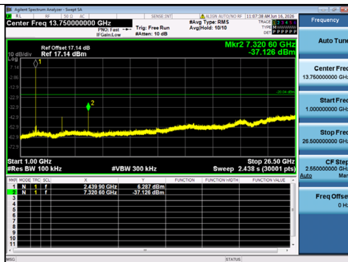
BLE_1M-Ant1-2440-1000~26500-PASS
