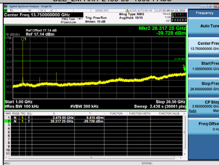
BLE_2M-Ant1-2480-1000~26500-PASS
