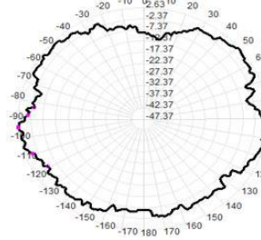
5790.0MHz Total(E2), Max= 2.63dBi
