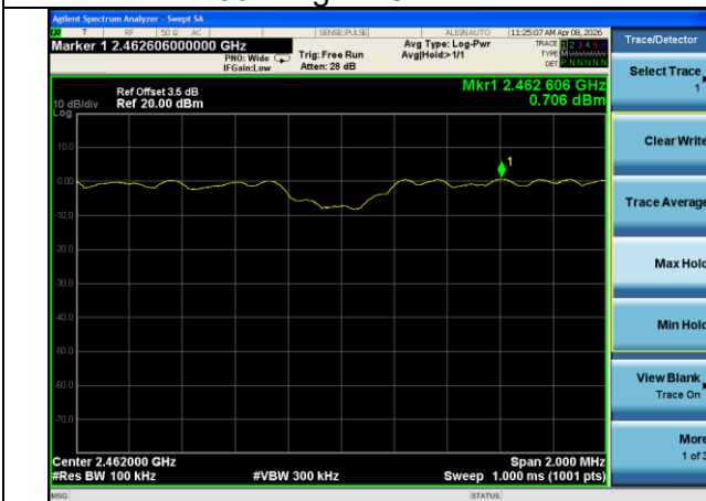
802.11g on Channel 11
