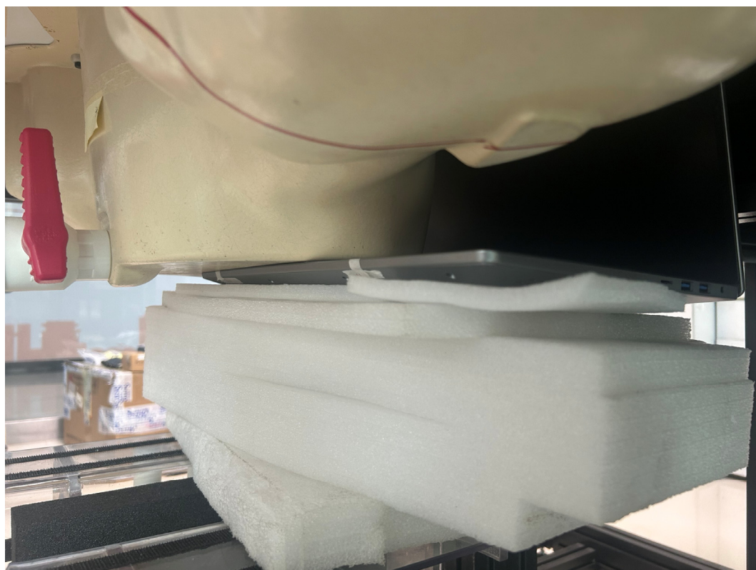
AUX ANT - Limb Front Setup Photo (0 mm)
