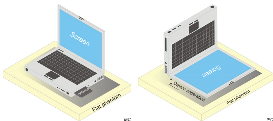
b) Portable computer with external-antenna plug-in radio card (left side) or with internal antenna located in screen section (right side)
