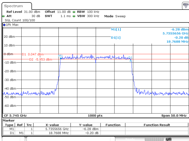
802.11ax20_5745MHz_RU_Full_Chain 0
