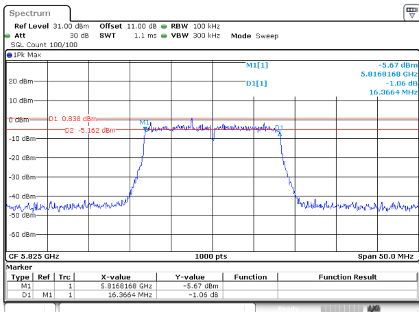
802.11a_5825MHz_Chain 0
