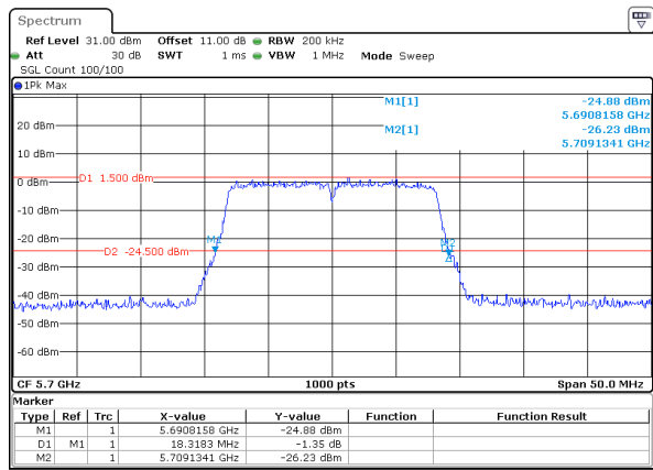
802.11a_5700MHz_Chain 0
