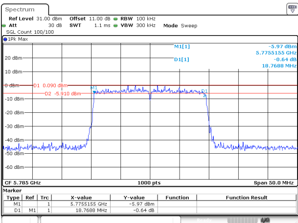
802.11ax20_5785MHz_RU_Full_Chain 0
