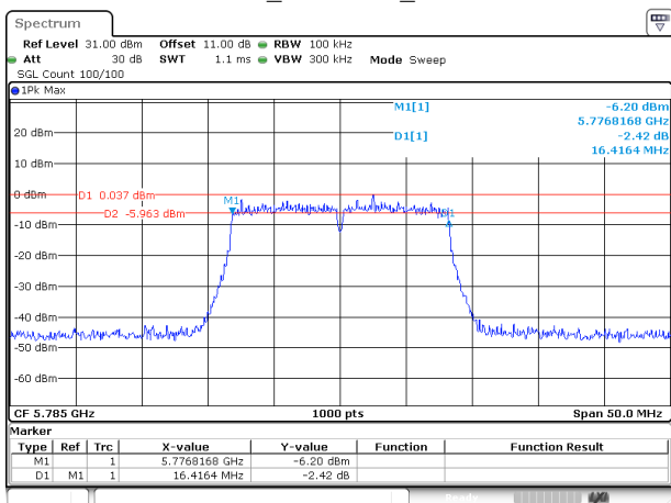
802.11a_5785MHz_Chain 1
