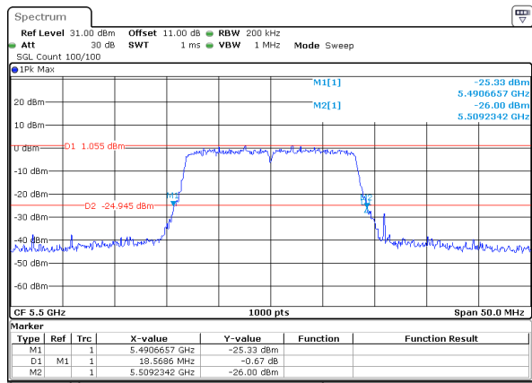
802.11a_5500MHz_Chain 0
