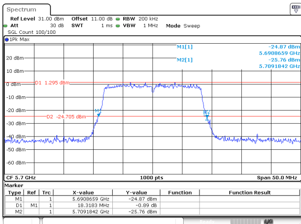
802.11a_5700MHz_Chain 1
