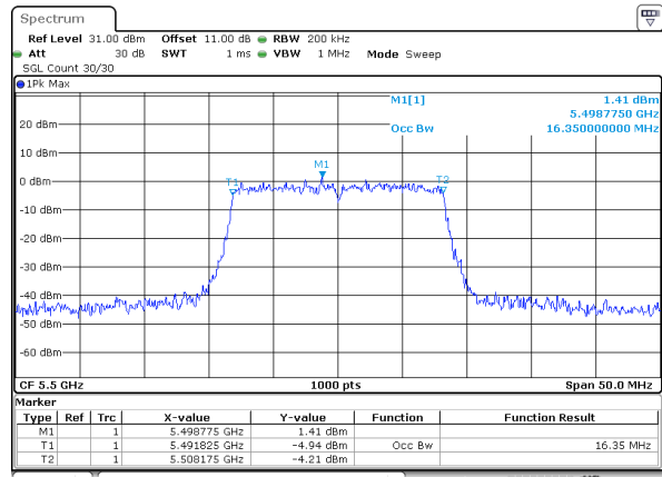
802.11a_5500MHz_Chain 0
