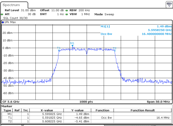
802.11a_5600MHz_Chain 0
