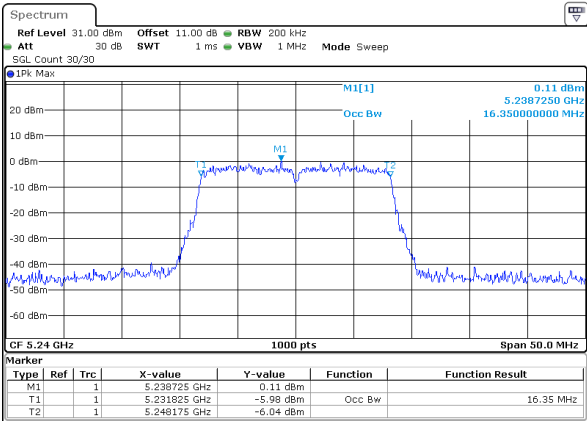
802.11a_5240MHz_Chain 0
