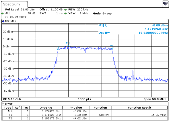
802.11a_5180MHz_Chain 1
