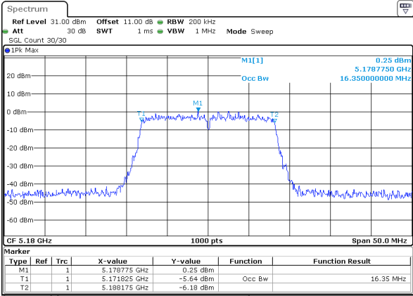
802.11a_5180MHz_Chain 0
