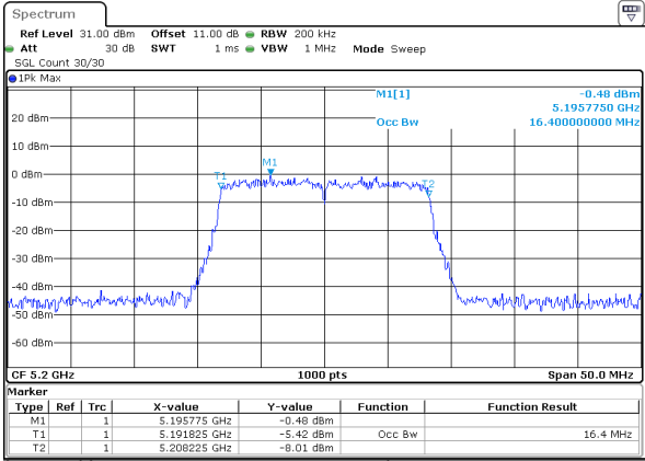
802.11a_5200MHz_Chain 0
