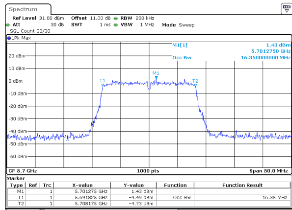
802.11a_5700MHz_Chain 0
