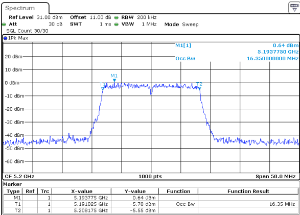
802.11a_5200MHz_Chain 1
