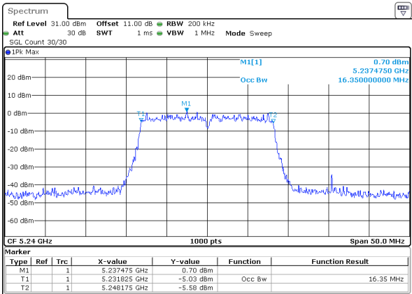
802.11a_5240MHz_Chain 1
