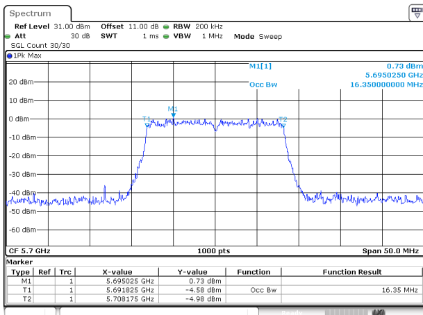
802.11a_5700MHz_Chain 1
