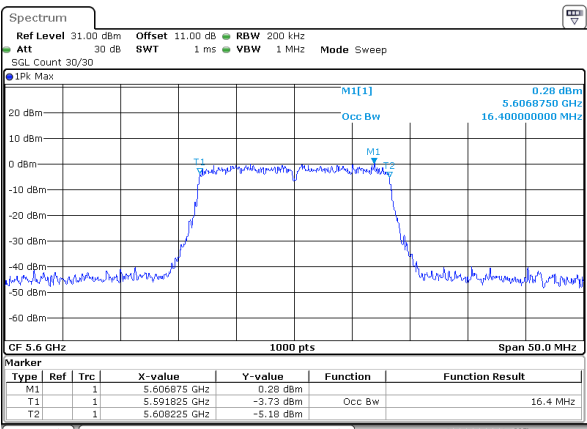
802.11a_5600MHz_Chain 1
