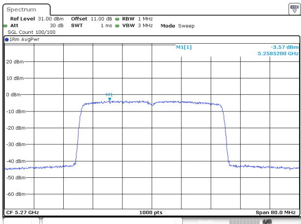
802.11ax40_5270MHz_RU_Full_Chain 1
