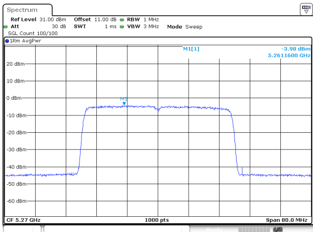
802.11ax40_5270MHz_RU_Full_Chain 0
