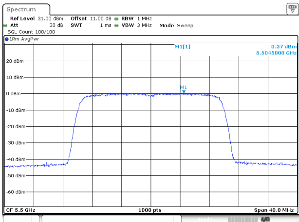
802.11ax20_5500MHz_RU_Full_Chain 1
