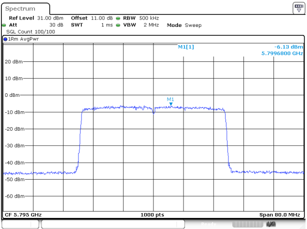
802.11ax40_5795MHz_RU_Full_Chain 1
