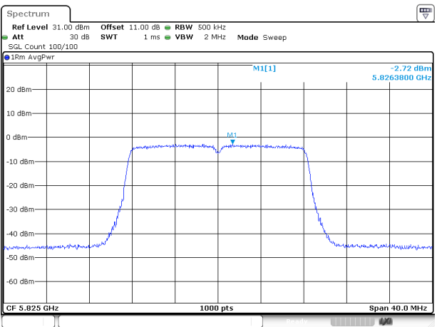
802.11a_5825MHz_Chain 1
