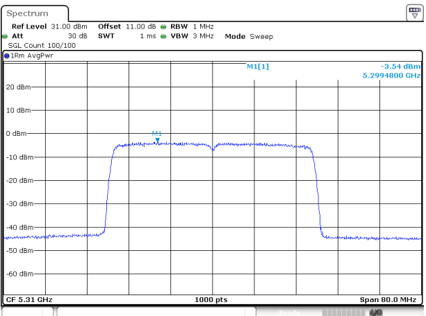
802.11ax40_5310MHz_RU_Full_Chain 0
