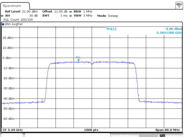
802.11ax40_5590MHz_RU_Full_Chain 0
