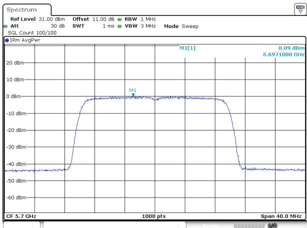
802.11ax20_5700MHz_RU_Full_Chain 0
