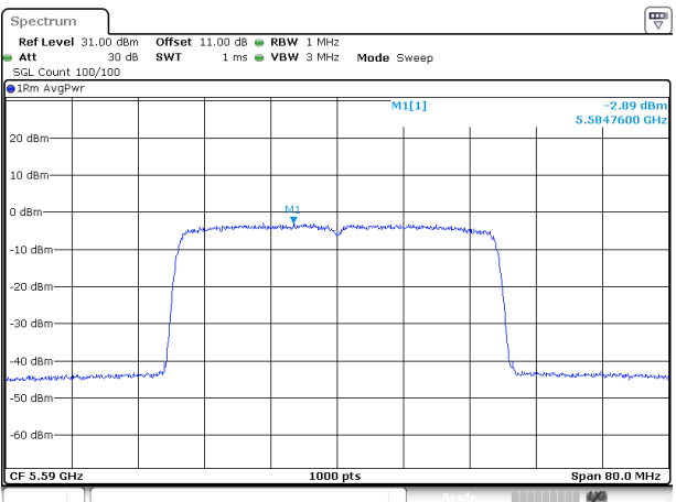
802.11ax40_5590MHz_RU_Full_Chain 1
