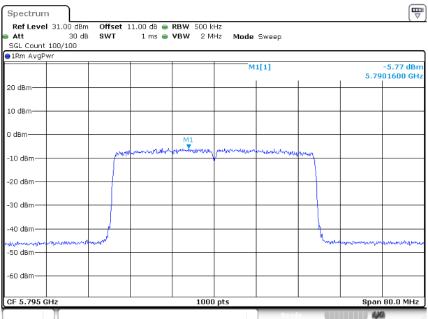
802.11ax40_5795MHz_RU_Full_Chain 0
