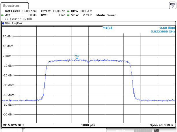
802.11ax20_5825MHz_RU_Full_Chain 1
