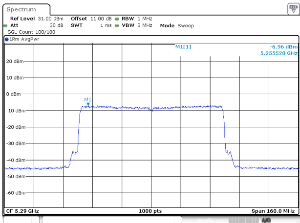
802.11ax80_5290MHz_RU_Full_Chain 0
