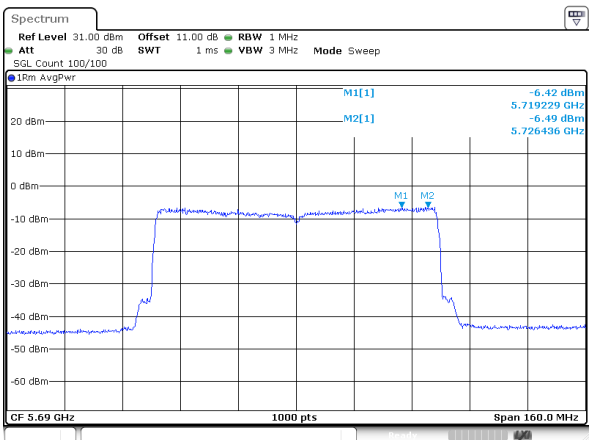
802.11ax80_5690MHz_RU_Full_Chain 1
