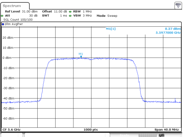
802.11ax20_5600MHz_RU_Full_Chain 1
