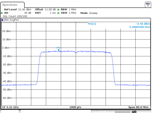
802.11ax40_5310MHz_RU_Full_Chain 1
