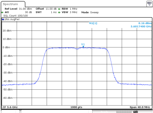
802.11a_5600MHz_Chain 1
