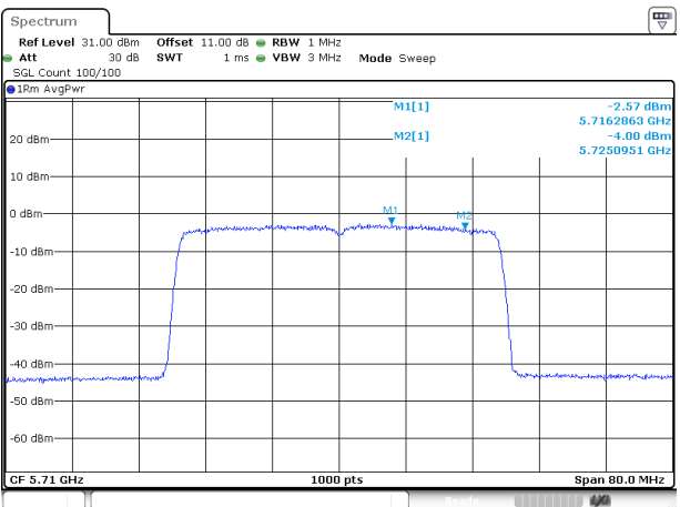
802.11ax40_5710MHz_RU_Full_Chain 0
