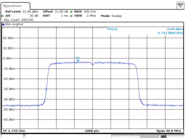
802.11ax20_5745MHz_RU_Full_Chain 1
