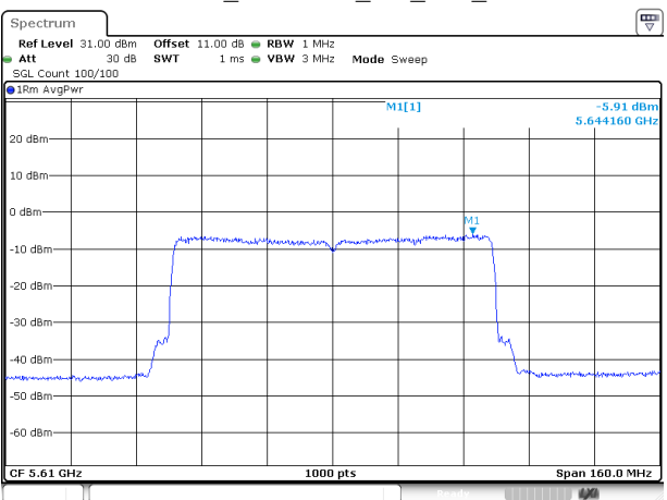
802.11ax80_5610MHz_RU_Full_Chain 0
