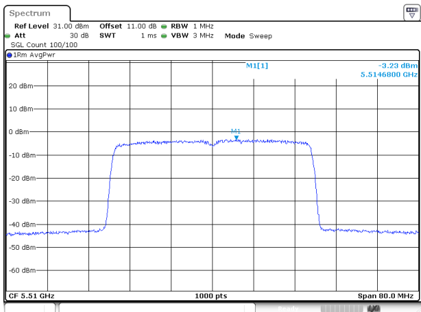
802.11ax40_5510MHz_RU_Full_Chain 0
