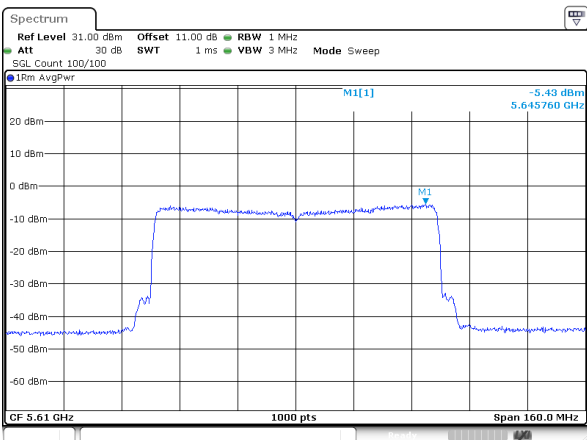
802.11ax80_5610MHz_RU_Full_Chain 1
