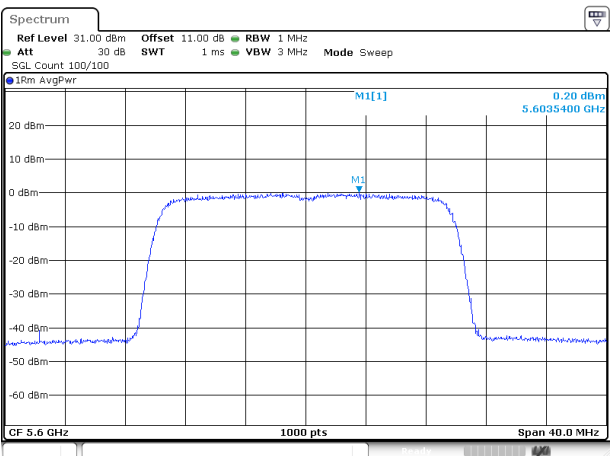
802.11ax20_5600MHz_RU_Full_Chain 0
