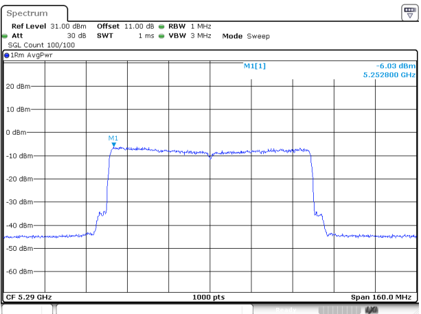
802.11ax80_5290MHz_RU_Full_Chain 1
