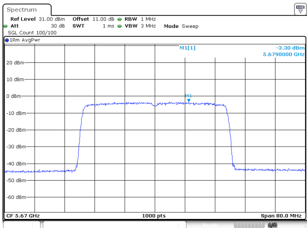
802.11ax40_5670MHz_RU_Full_Chain 0
