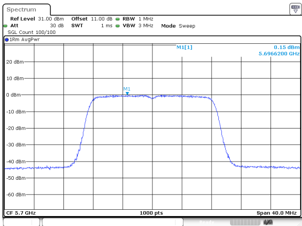
802.11a_5700MHz_Chain 1
