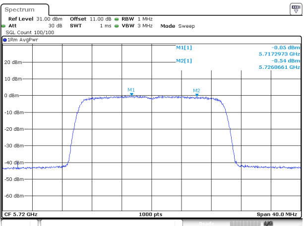
802.11ax20_5720MHz_RU_Full_Chain 1
