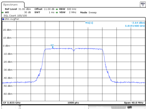
802.11a_5825MHz_Chain 0
