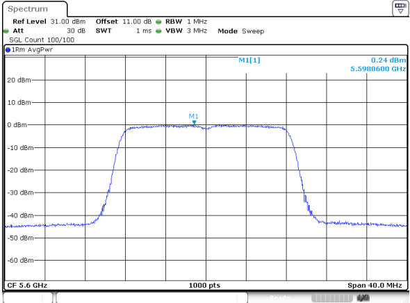
802.11a_5600MHz_Chain 0
