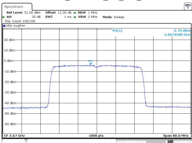
802.11ax40_5670MHz_RU_Full_Chain 1
