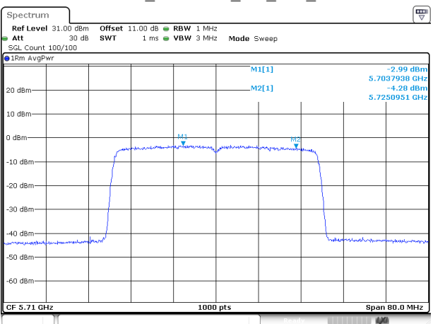
802.11ax40_5710MHz_RU_Full_Chain 1
