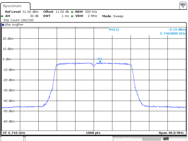
802.11a_5745MHz_Chain 1
