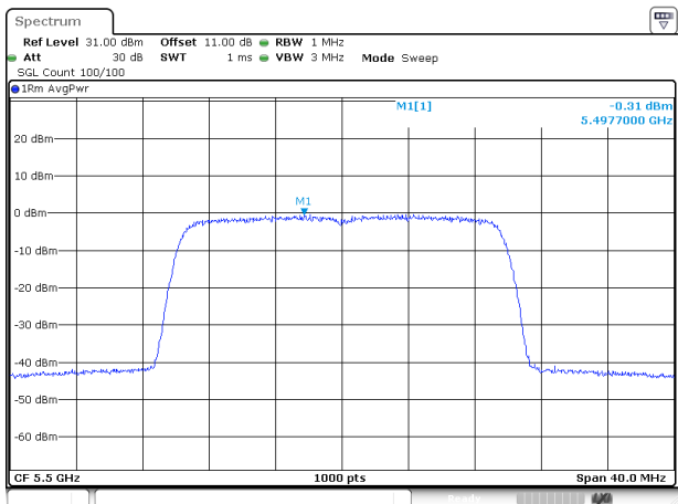
802.11ax20_5500MHz_RU_Full_Chain 0
