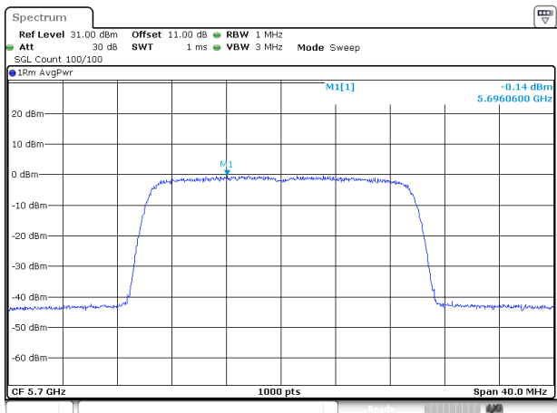
802.11ax20_5700MHz_RU_Full_Chain 1
