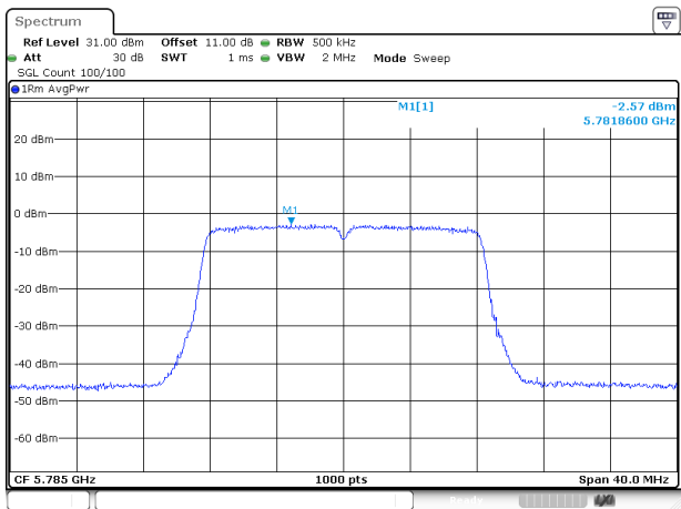
802.11a_5785MHz_Chain 1
