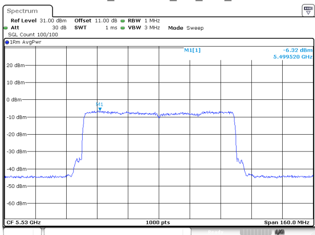
802.11ax80_5530MHz_RU_Full_Chain 0
