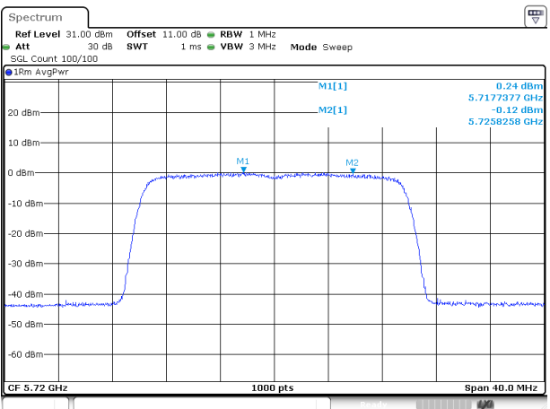
802.11ax20_5720MHz_RU_Full_Chain 0
