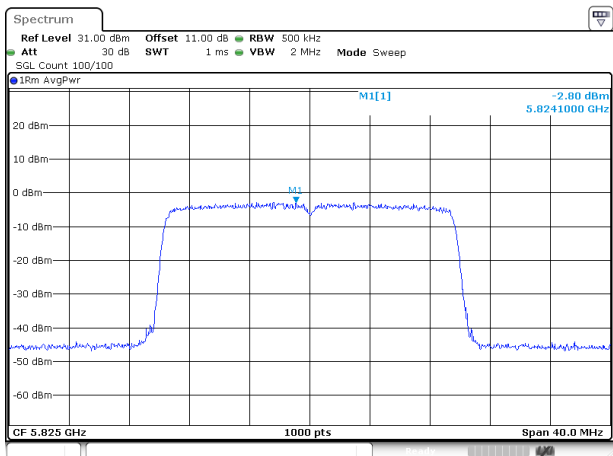
802.11ax20_5825MHz_RU_Full_Chain 0
