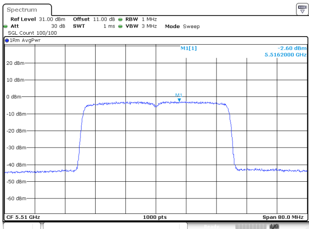
802.11ax40_5510MHz_RU_Full_Chain 1
