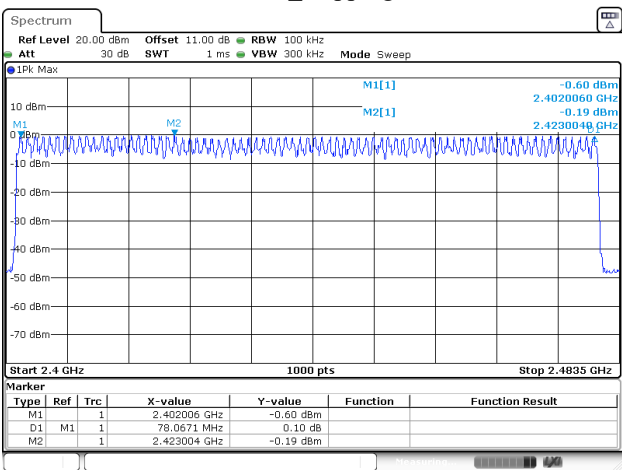
3DH1_Hopping
