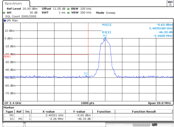
2DH1_Low
