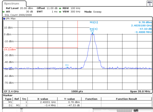
DH1_Low
